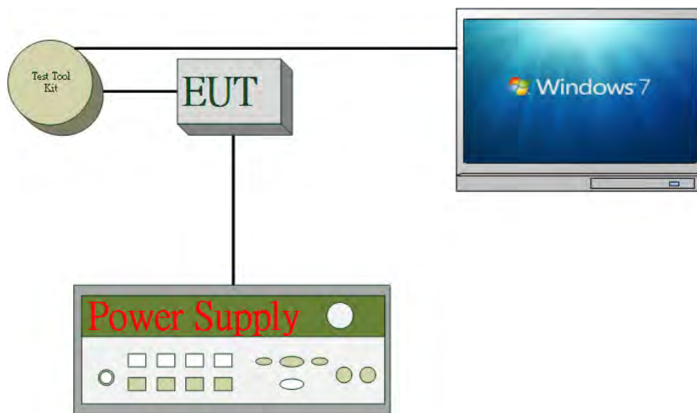
Fig. 2-1 Radiated Emission & Conducted (Antenna Port) Configuration
