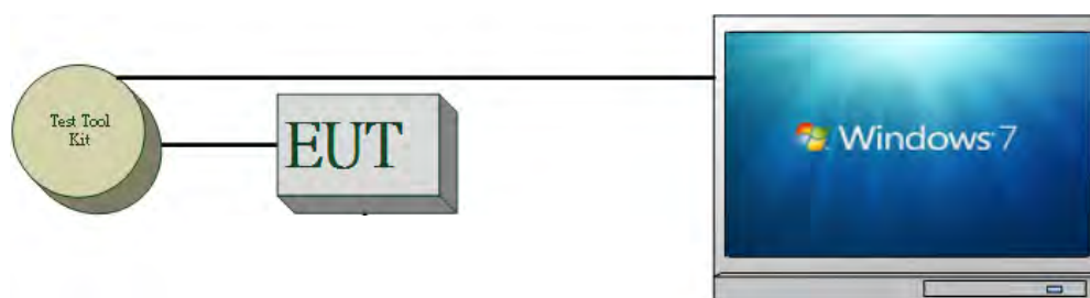
Fig. 2-1 AC Power Line Conducted Emission Configuration
