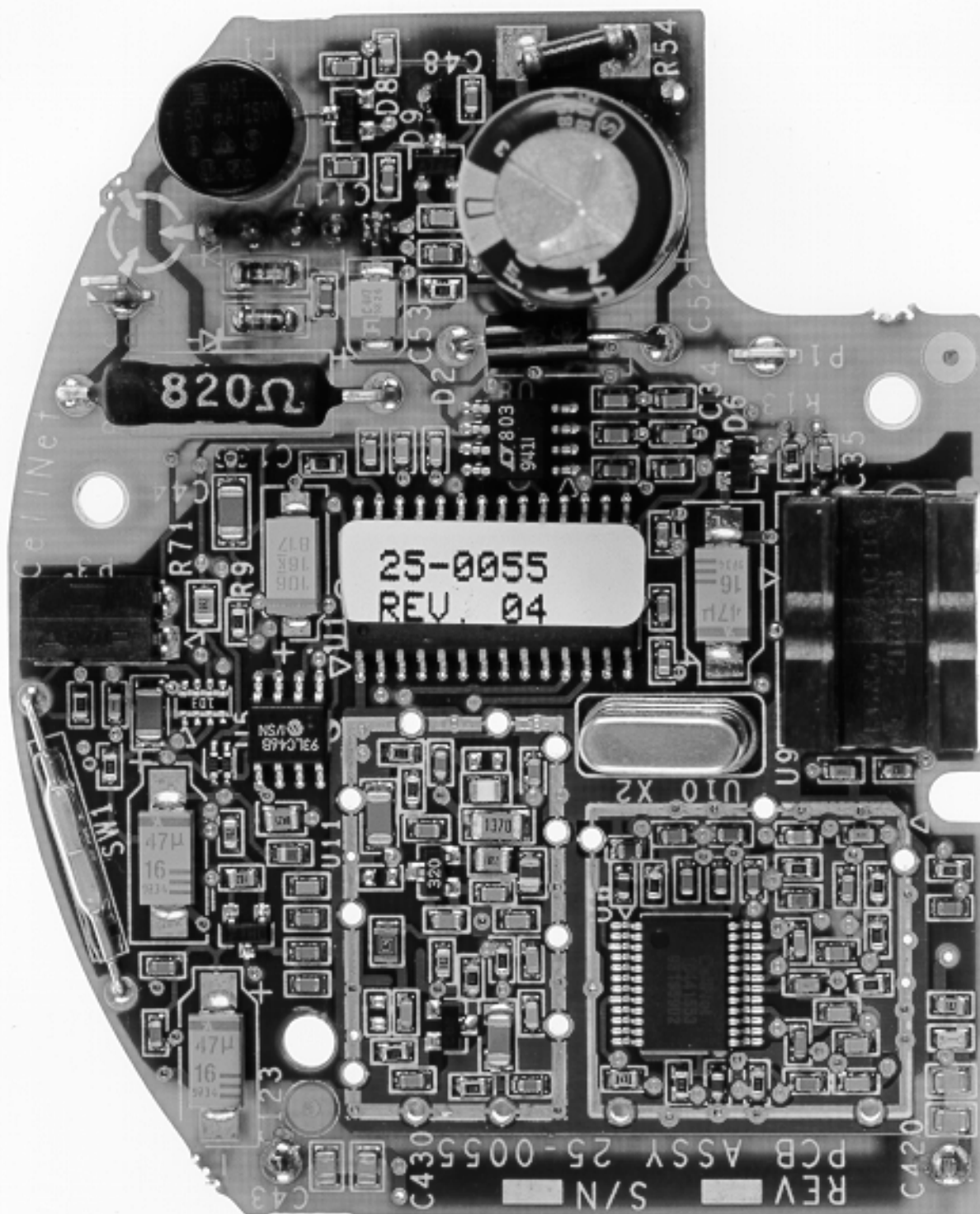
Cellnet Data Systems FCC ID: H6NCMM1102 PCB w/o covers - Top View
