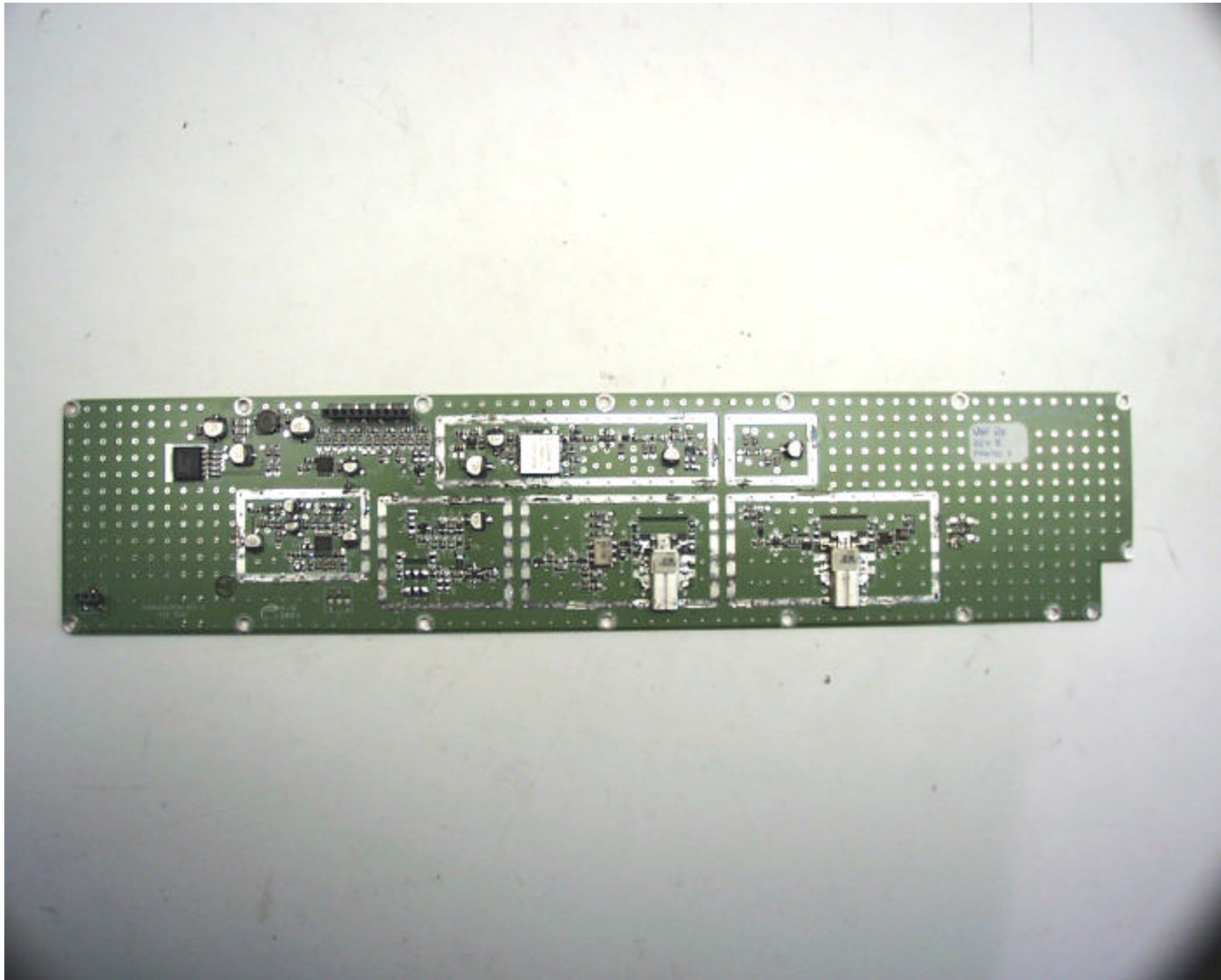
Exhibit 12 - Photograph # 14 (Internal Photos of Kaval LINKnet OFR400 Module)
