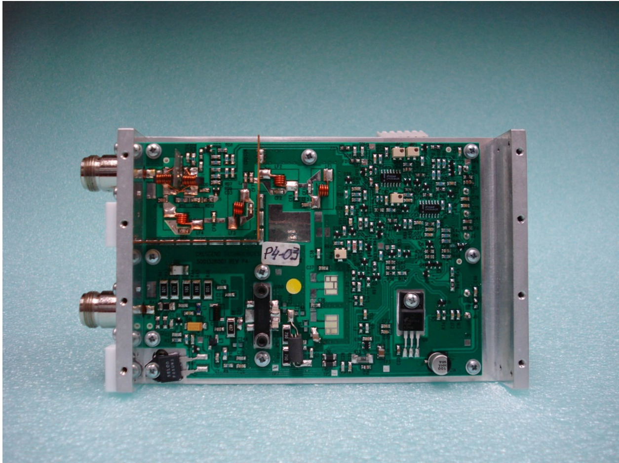
4 - Amp Board Front
