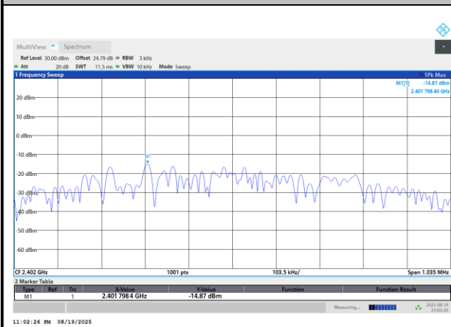
Power Density (dBm/3kHz) Plot Channel 0
