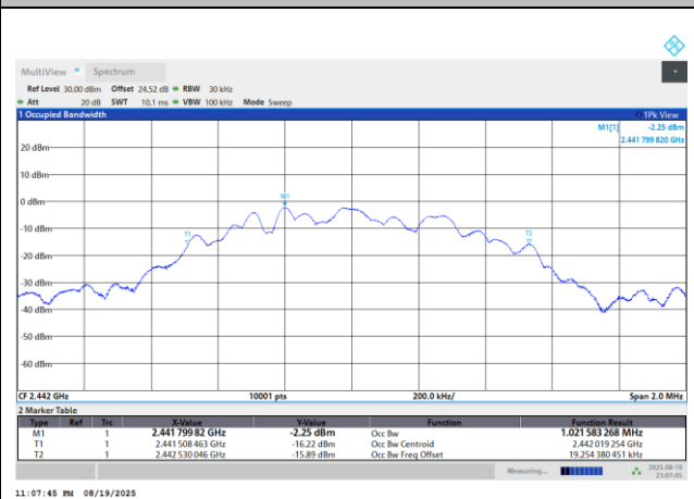
99% Occupied Bandwidth Plot on Channel 20
