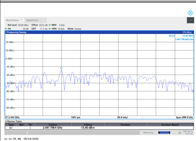
Power Density (dBm/3kHz) Plot Channel 20
