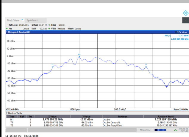
99% Occupied Bandwidth Plot on Channel 39
