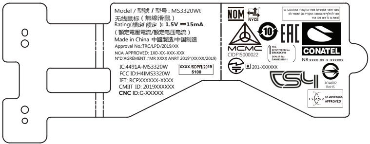
back side layout scale:1:1
