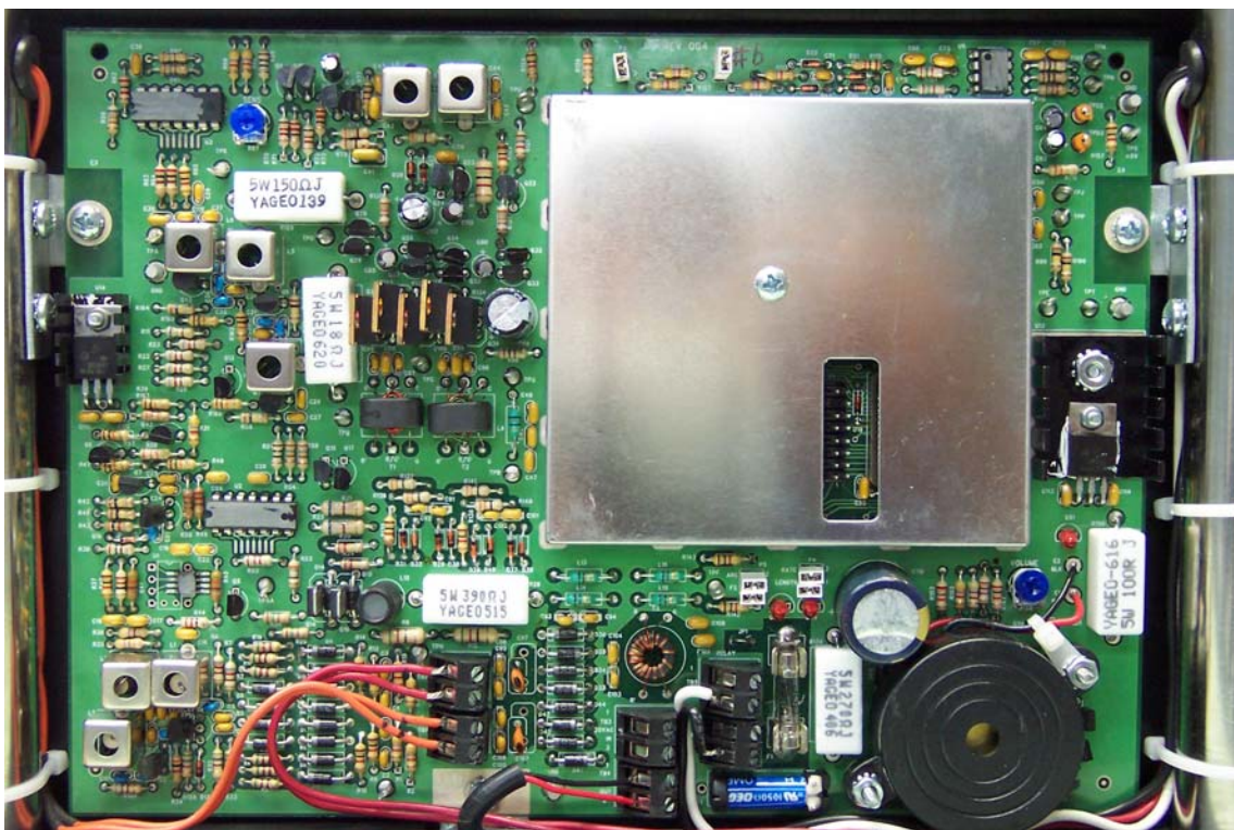
PCB Front View Shield Can Attached
