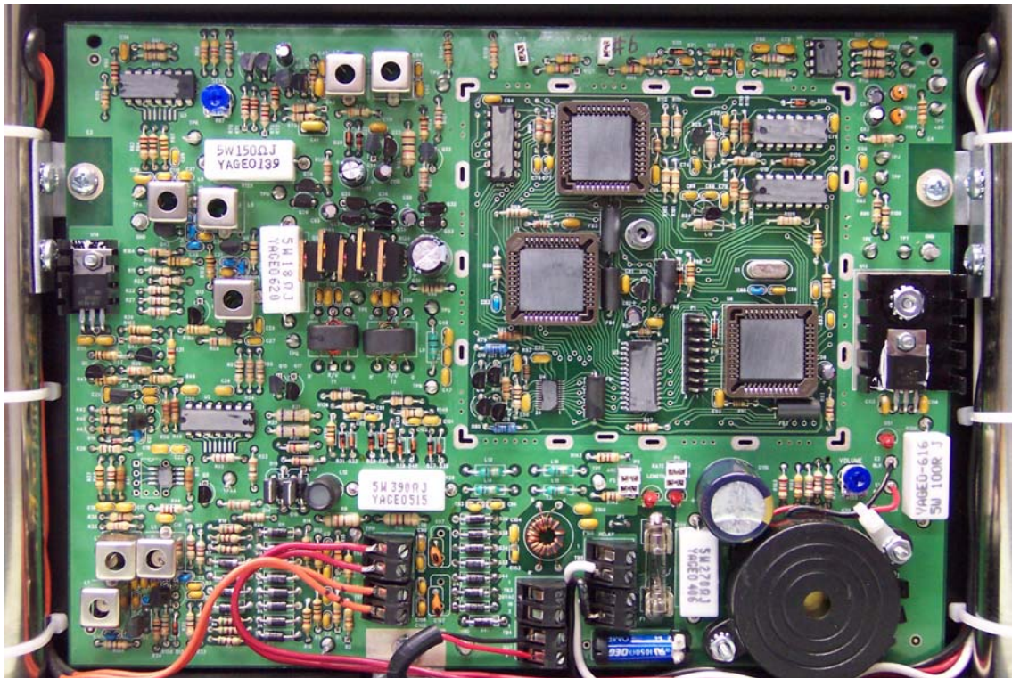
PCB Front View Shield Can Removed
