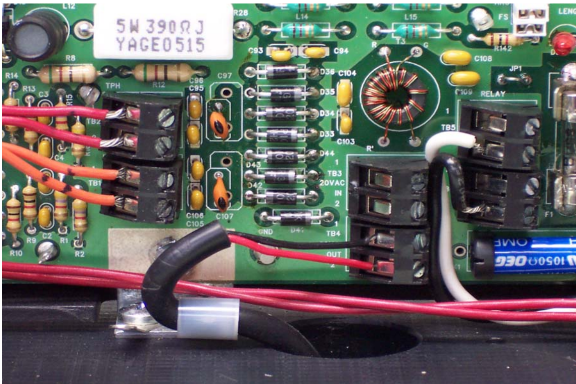
PCB Front Terminal Block Connections
