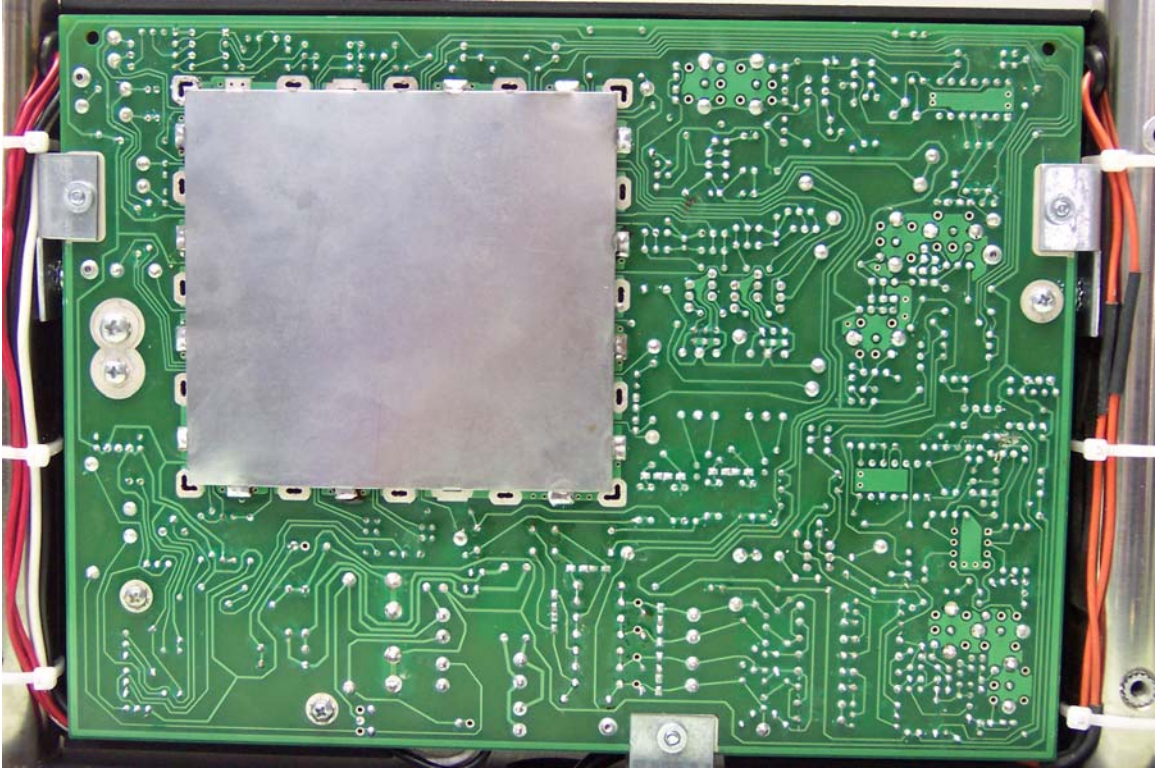
PCB Rear View Shield Cover Attached
