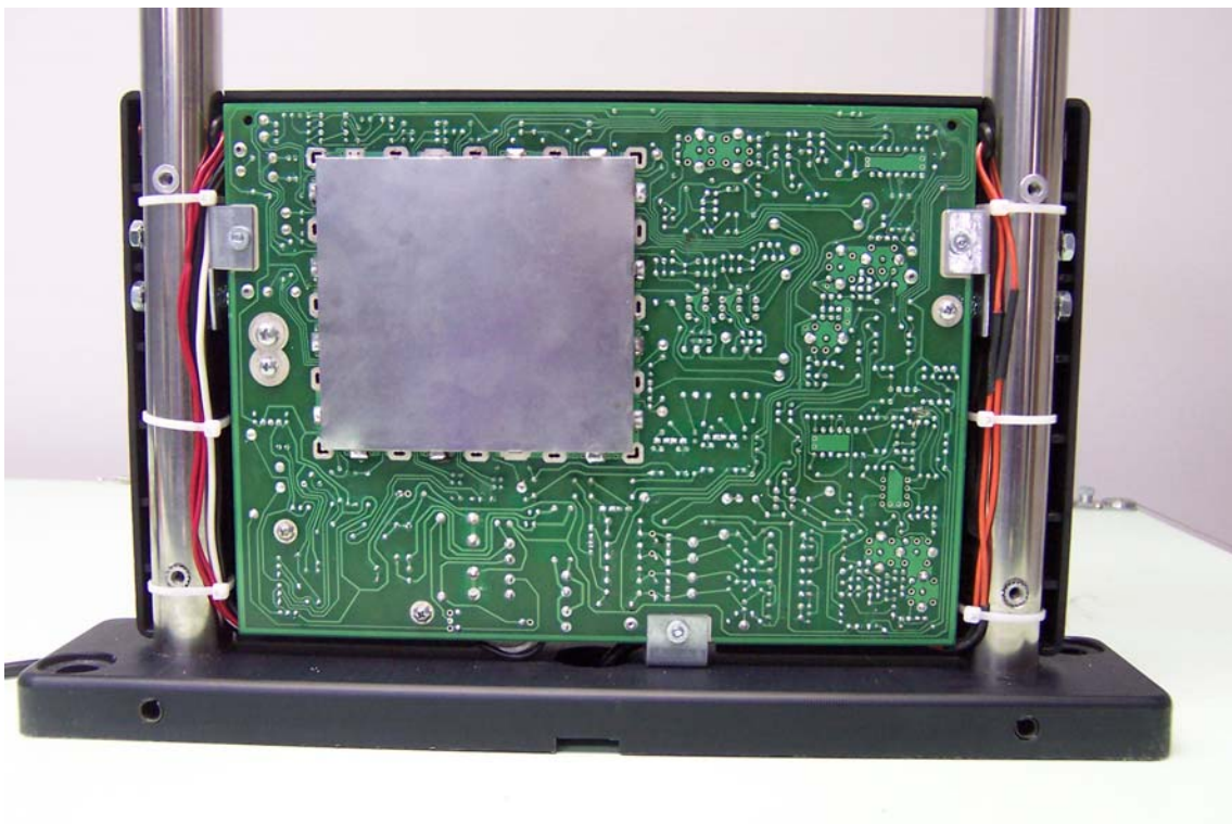
Rear View Plastic Cover Removed
