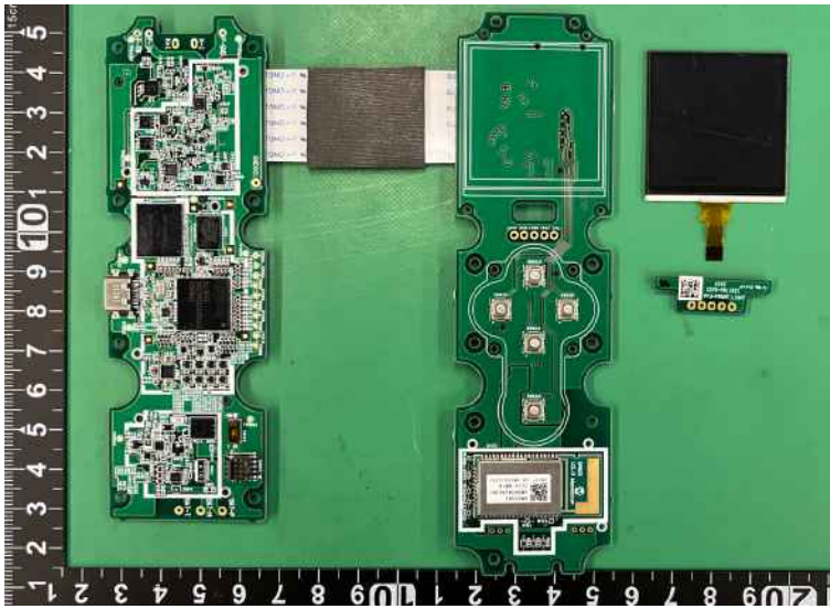
PCB Antenna (BT)
