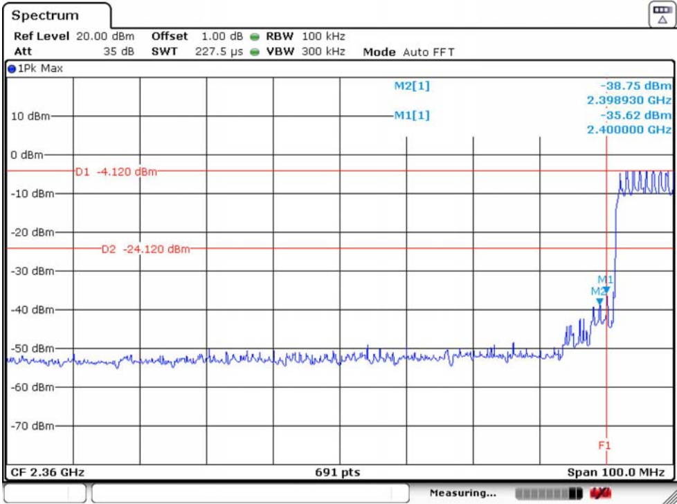
\pi/4 -DQPSK Low Channel Channel Hopping ON
