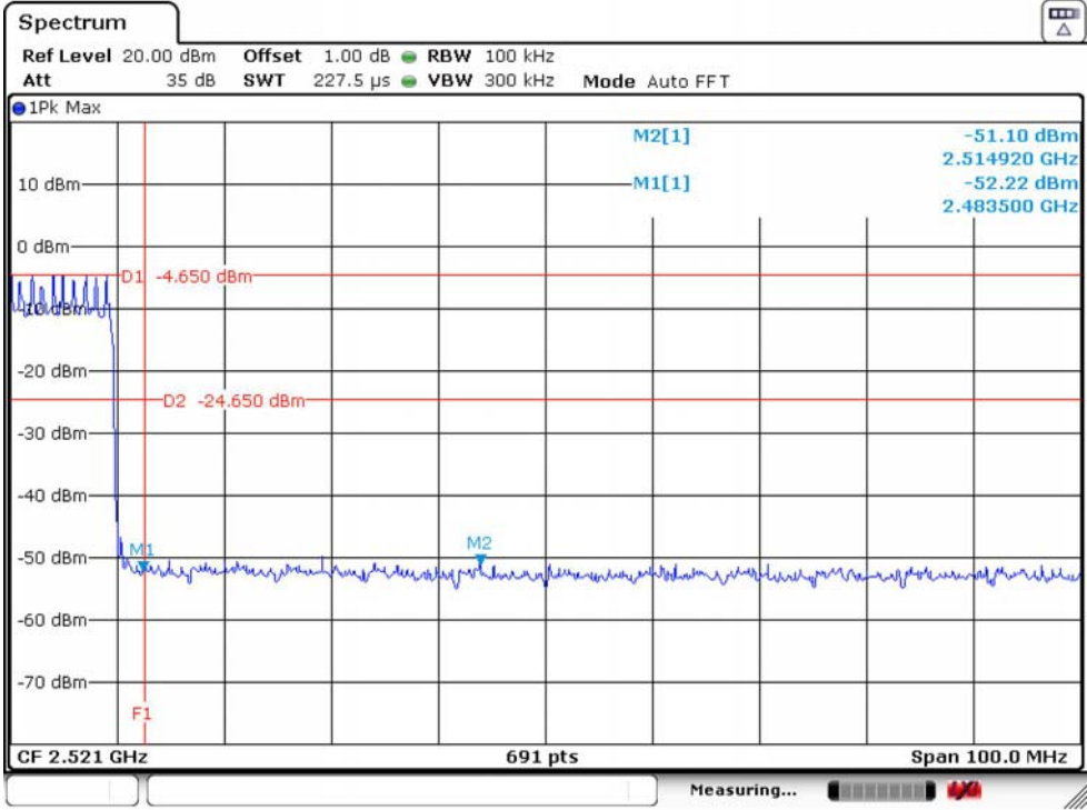
\pi/4 -DQPSK High Channel Hopping ON
