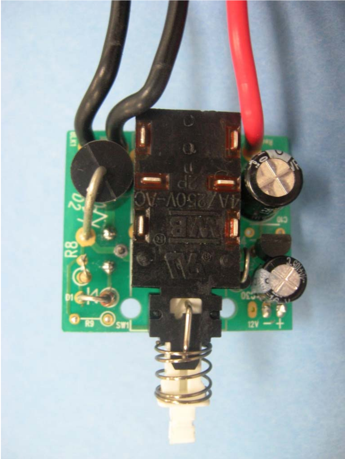
Switch Board – Top
