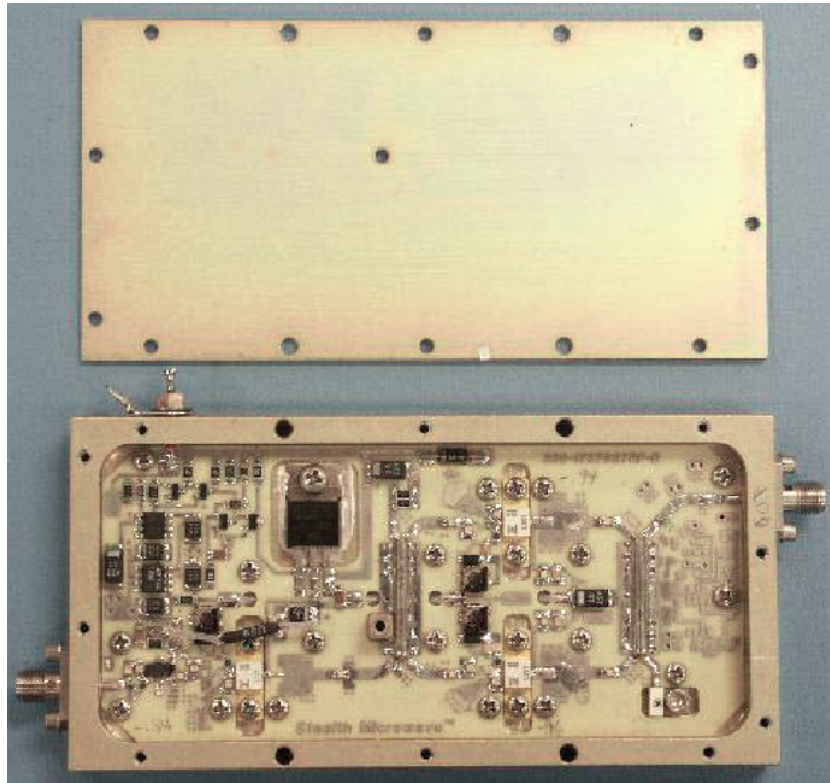
Stealth Microwave SM2025-42LS Power Amplifier In Housing
