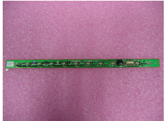
Soft-Touch Keyboard module
