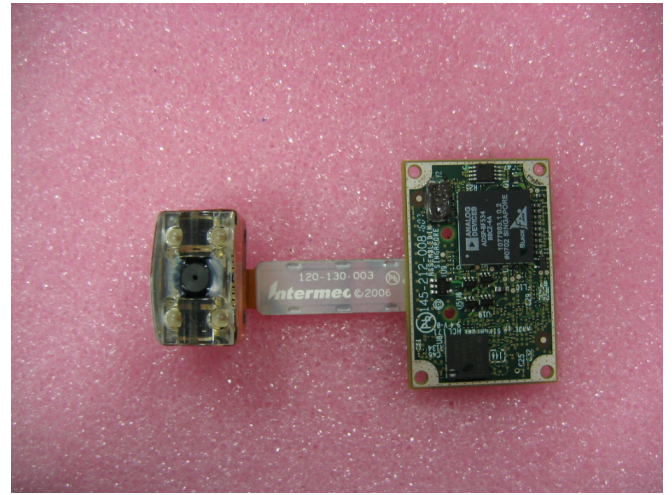
Barcode Reader Module Front side
