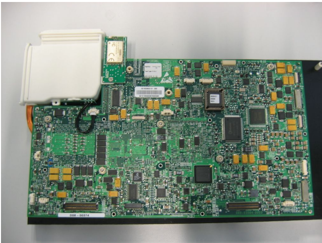
MB top view
