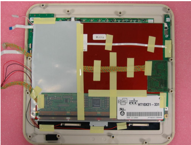
Front Assembly (Display LCD panel rear side)
