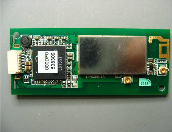
Photo 11 - USB BOARD front
