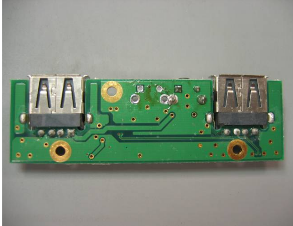
Photo 12 - USB BOARD front
