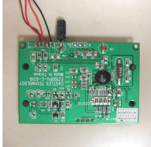
Photo 22 - Battery module (rear)
