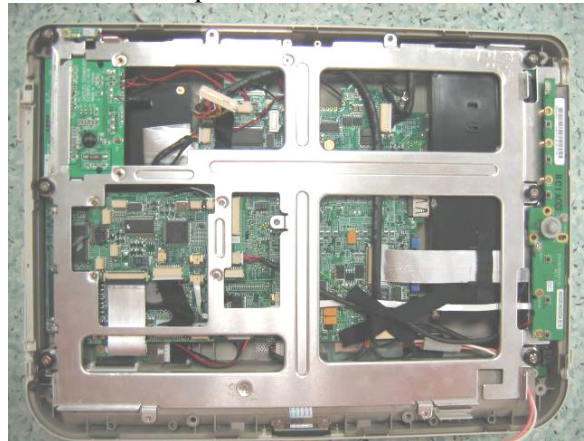
Photo 3 – LCD panel bracket
