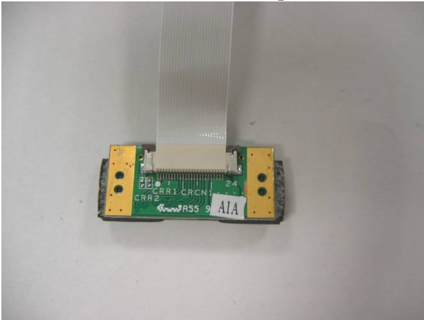
Photo 16 – Cradle connector adapter board (rear)
