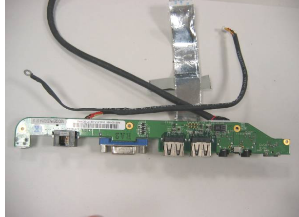
Photo 18 – I/O board connector (rear)
