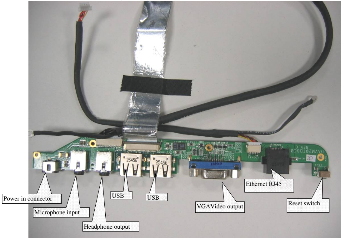
Photo 19 – I/O board connector (details)
