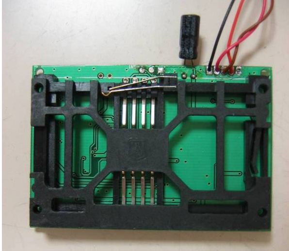
Photo 21– Battery module (front)
