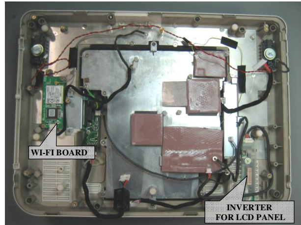
Photo 6 - LCD PANEL BRACKET
