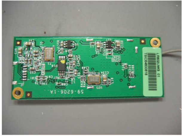
Photo 12 - USB BOARD front
