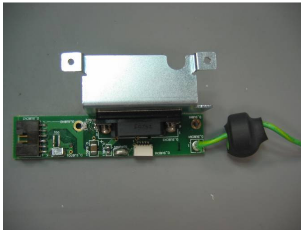
Photo 15 – CONTROL BOARD front
