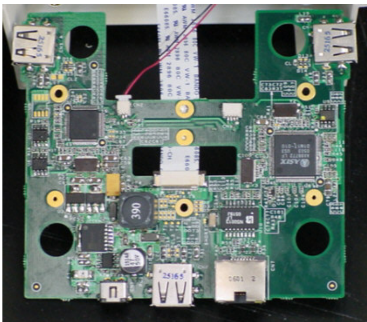
Figure 4: Docking station board
