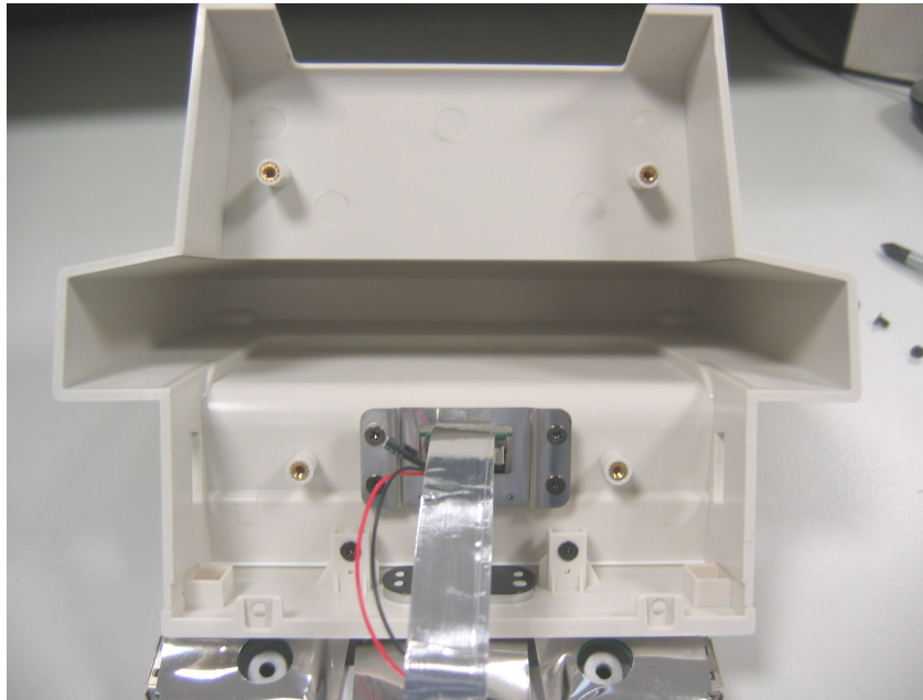
Figure : Detail of the led and connectors
