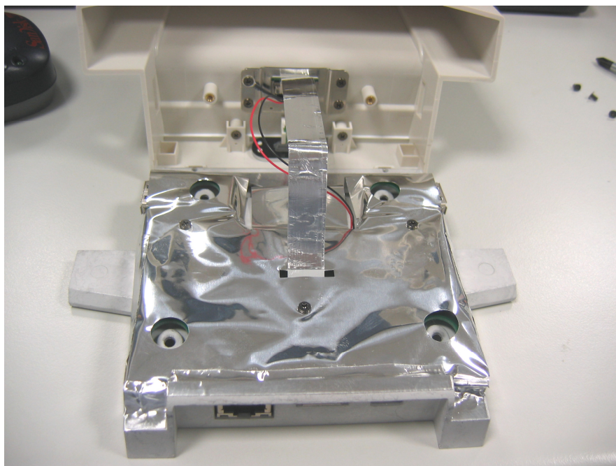
Figure 1: Overall view of the board
