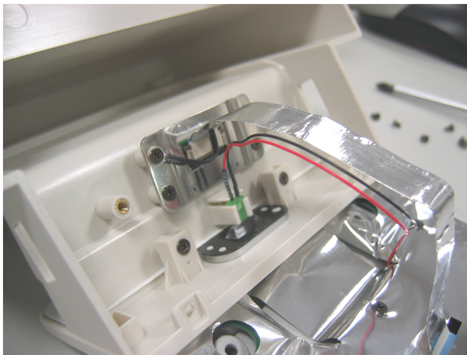
Figure 2 – Detail of the led and connectors
