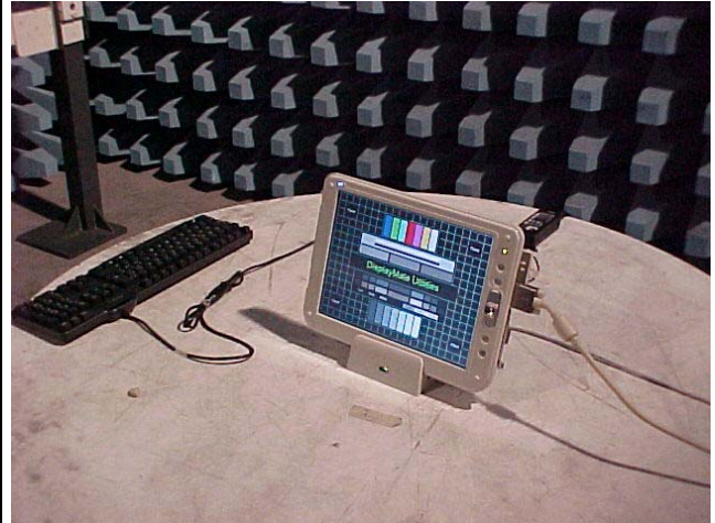
PHOTO 3 – SET-UP FOR EMISSION RADIATED TEST
