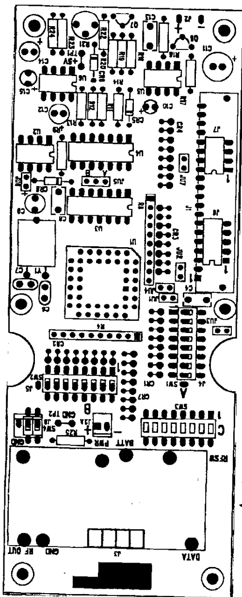
Control board
