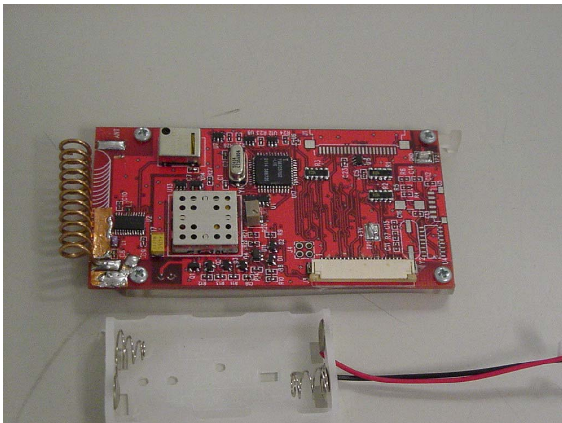
telePilot Internal Front Photo
