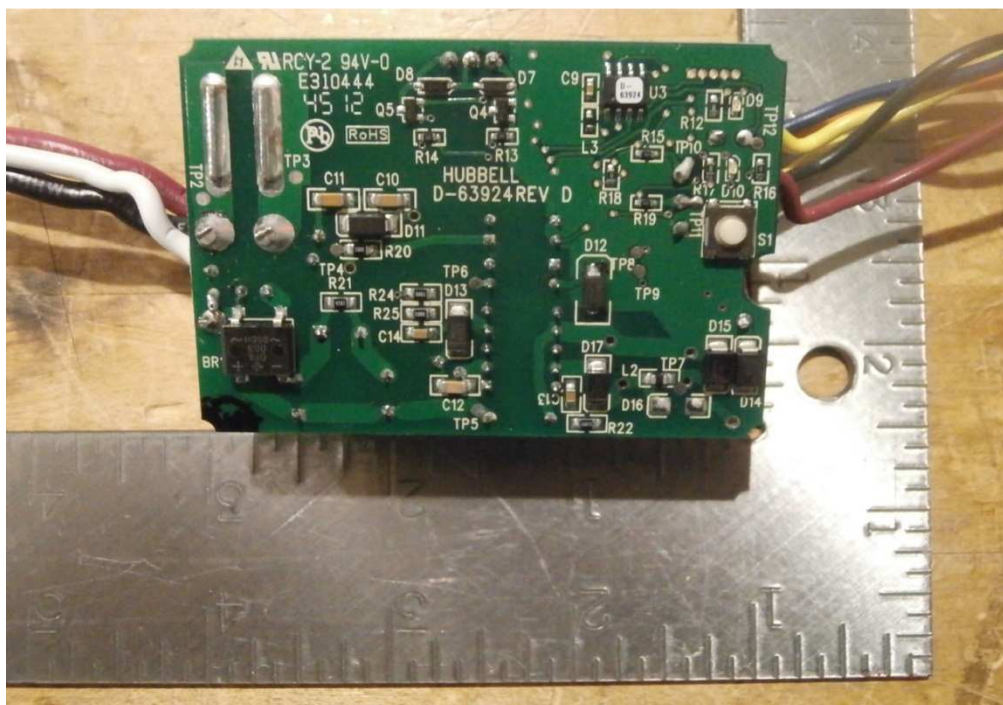
Main board bottom view
