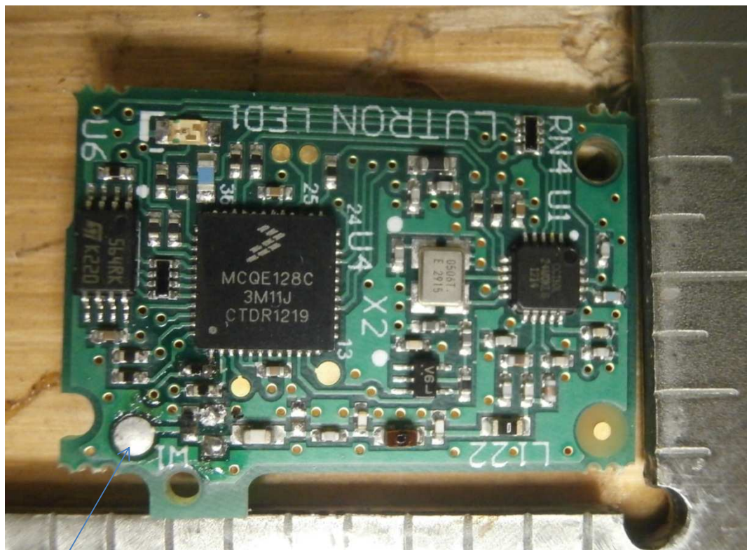
RF Board top view
