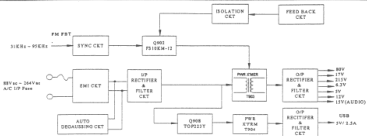
Figure 2 : Power supply block diagram
