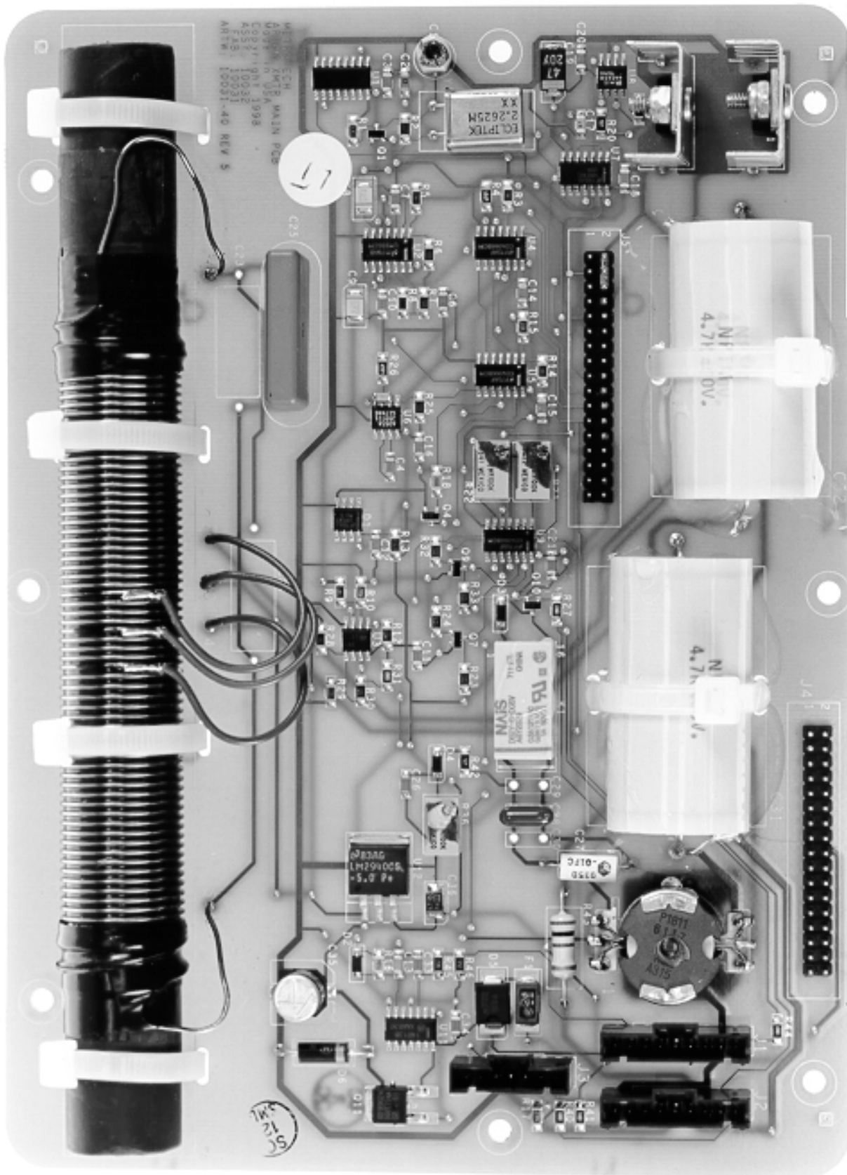
Metrotech FCC ID: GW6HNARROW Main Board - Top View
