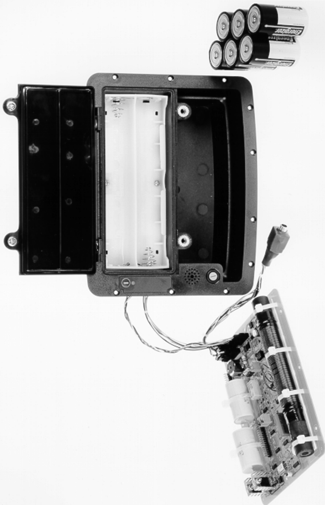
Metrotech FCC ID: GW6HNARROW Interior Exploded View
