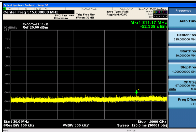
Band38-5MHz-16QAM-38225-1RB#0-30~1000MHz
