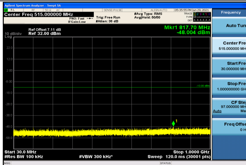
Band4-15MHz-QPSK-20325-1RB#0-30~1000MHz
