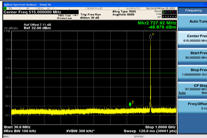
Band5-1.4MHz-QPSK-20643-1RB#0-30~1000MHz
