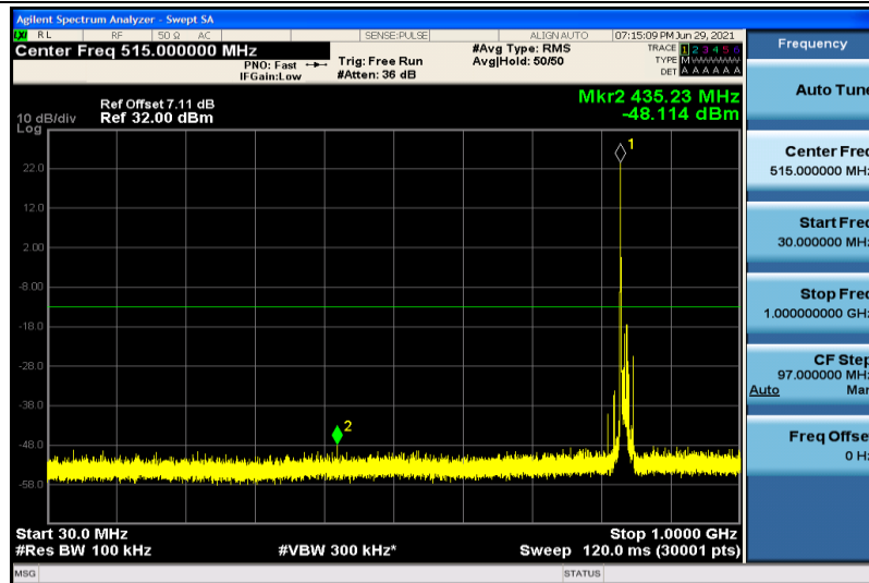
Band5-10MHz-16QAM-20525-1RB#0-30~1000MHz
