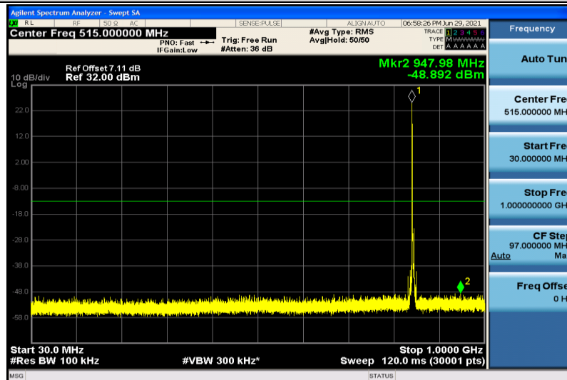
Band5-5MHz-16QAM-20625-1RB#0-30~1000MHz
