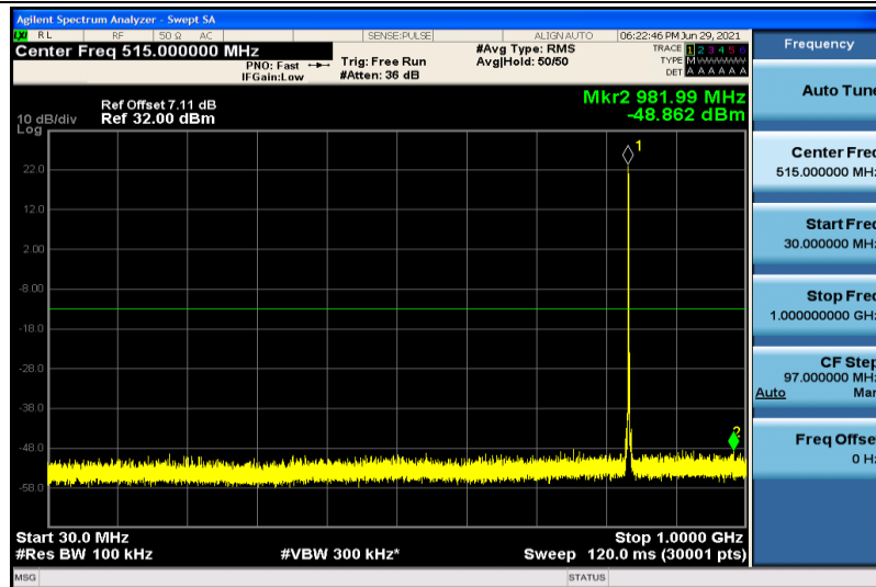
Band5-1.4MHz-QPSK-20525-1RB#0-30~1000MHz
