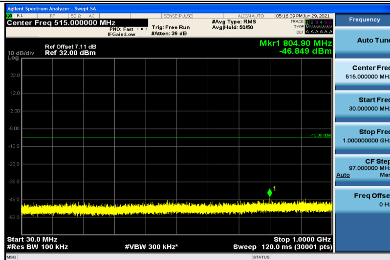
Band4-10MHz-QPSK-20350-1RB#0-30~1000MHz
