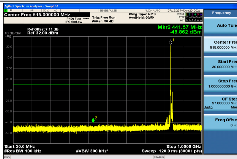
Band5-10MHz-16QAM-20600-1RB#0-30~1000MHz
