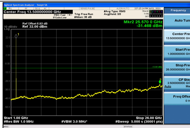
Band2-15MHz-QPSK-18675-1RB#0-1000~26000MHz
