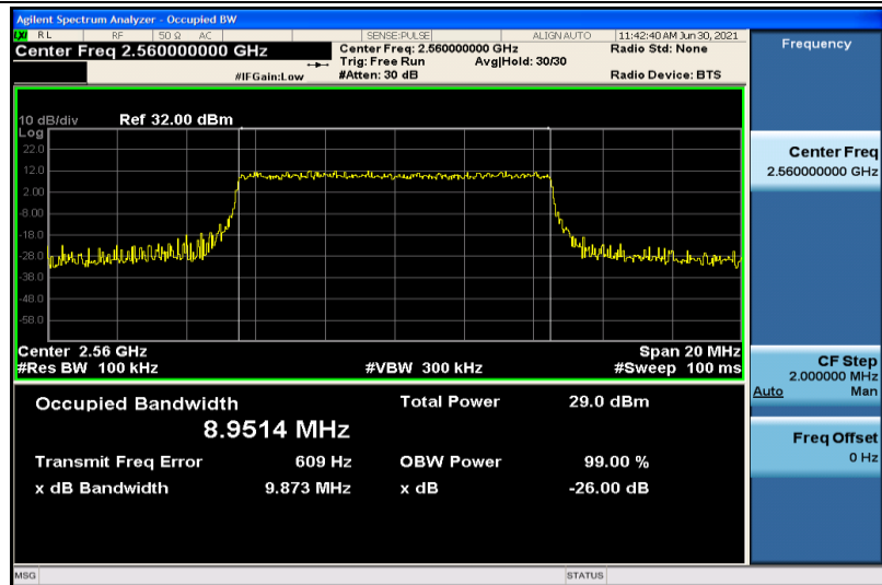
Band41-10MHz-QPSK-40290-50RB#0-8.9514
