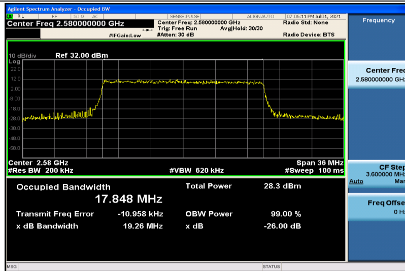
Band38-20MHz-16QAM-37850-100RB#0-17.848
