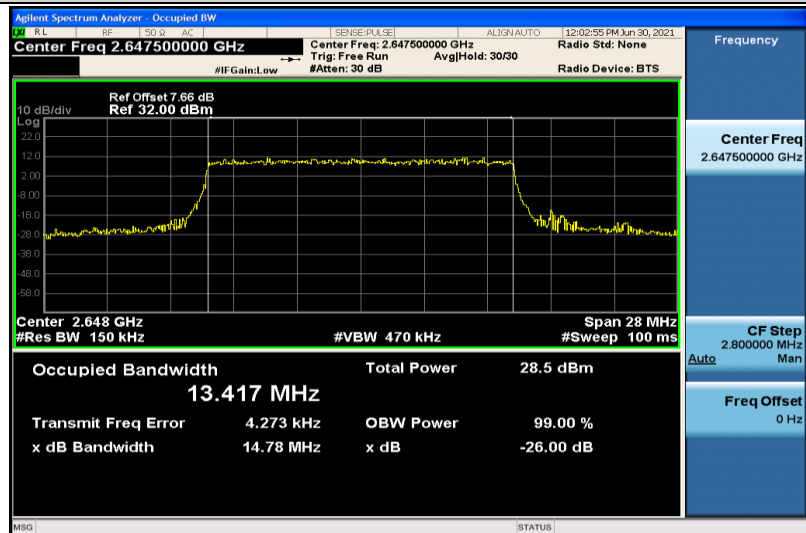
Band41-15MHz-QPSK-41165-75RB#0-13.417
