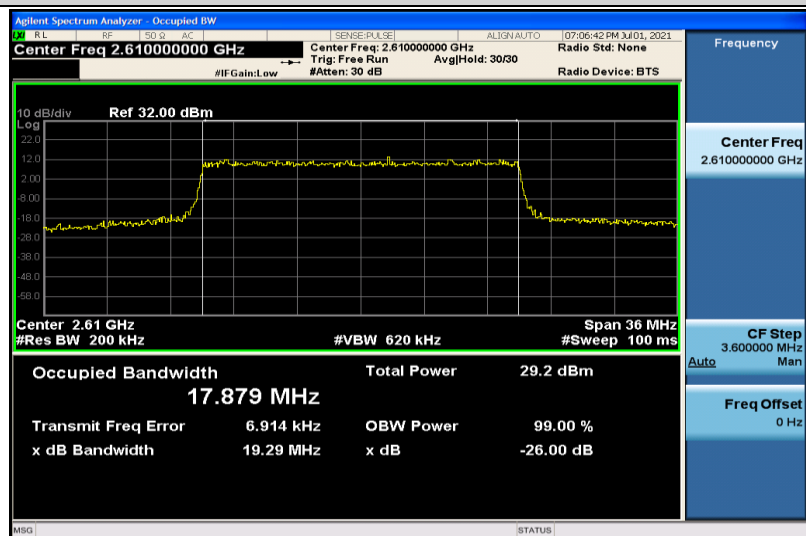
Band38-20MHz-QPSK-38150-100RB#0-17.879
