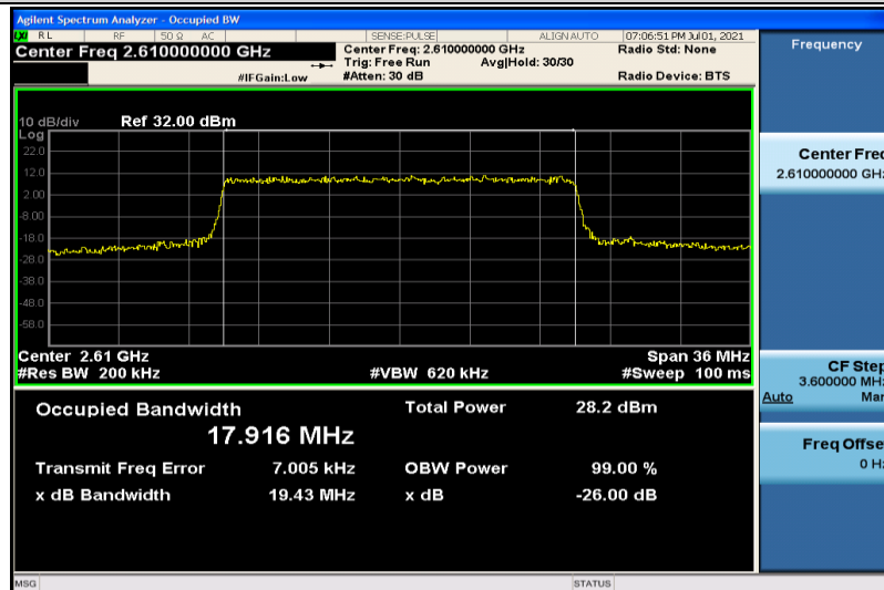
Band38-20MHz-16QAM-38150-100RB#0-17.916
