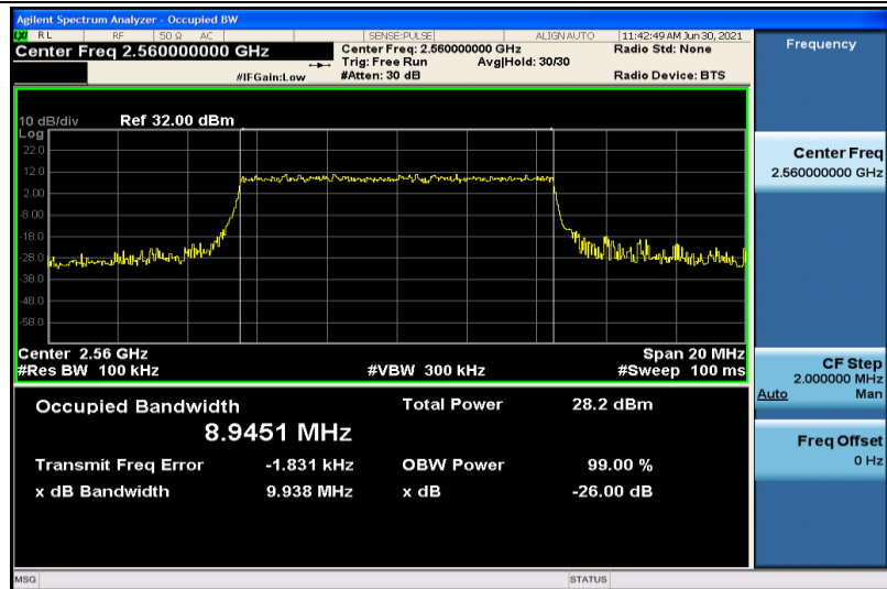
Band41-10MHz-16QAM-40290-50RB#0-8.9451
