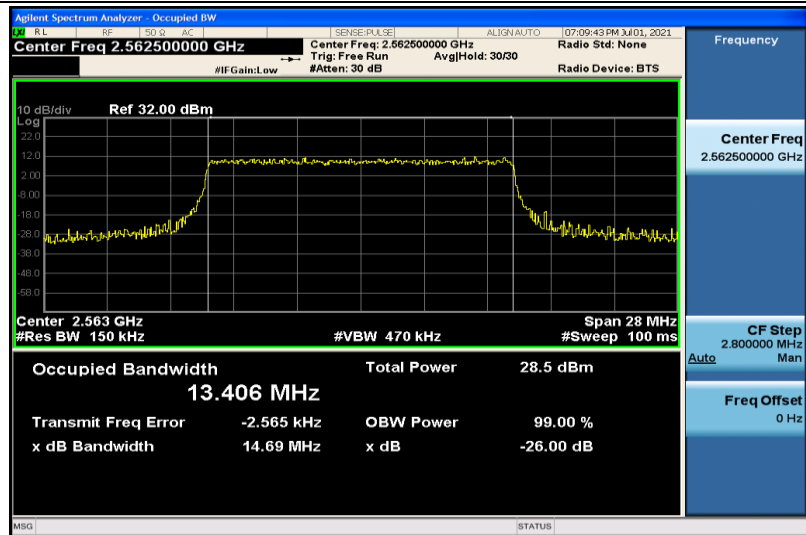
Band41-15MHz-QPSK-40315-75RB#0-13.406
