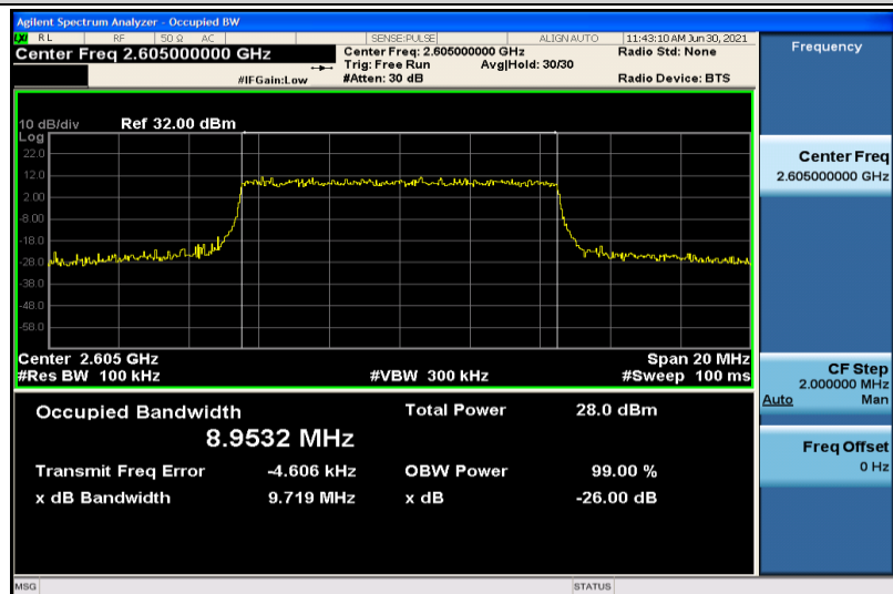
Band41-10MHz-16QAM-40740-50RB#0-8.9532
