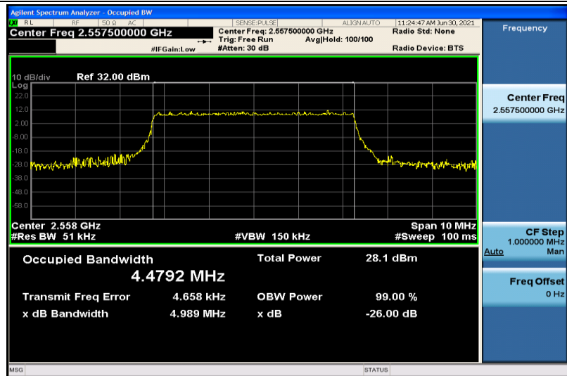
Band41-5MHz-16QAM-40265-25RB#0-4.4792
