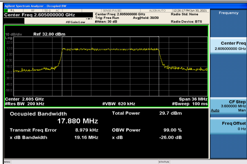
Band41-20MHz-QPSK-40740-100RB#0-17.880
