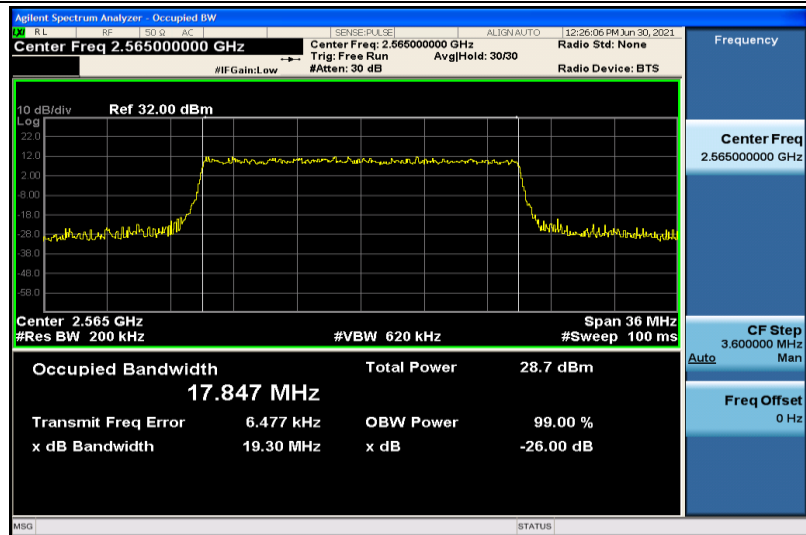
Band41-20MHz-16QAM-40340-100RB#0-17.847
