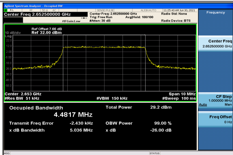
Band41-5MHz-QPSK-41215-25RB#0-4.4817
