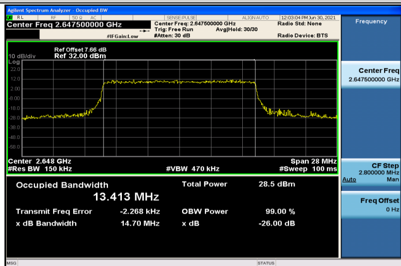
Band41-15MHz-16QAM-41165-75RB#0-13.413
