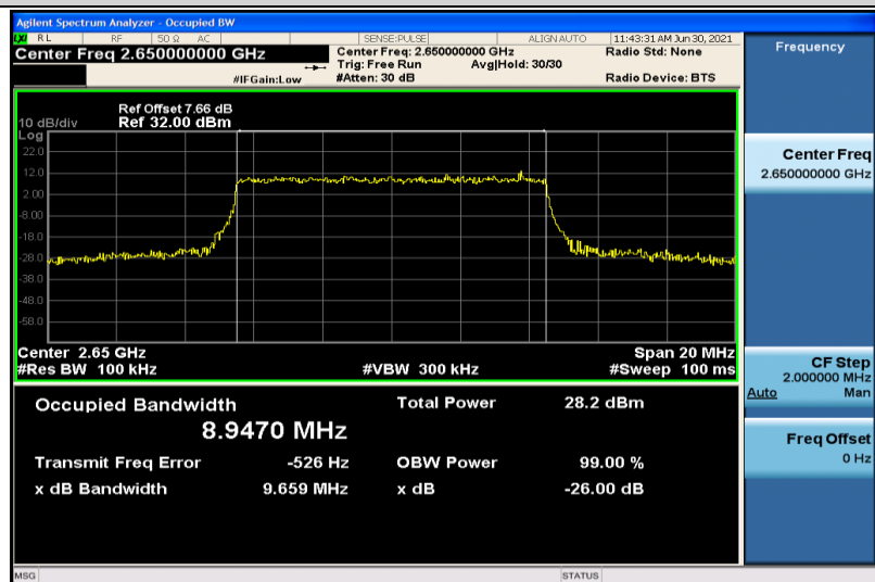
Band41-10MHz-16QAM-41190-50RB#0-8.9470
