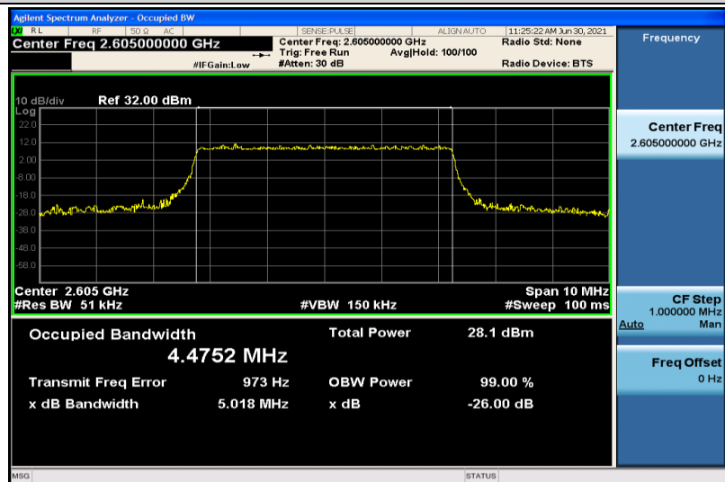
Band41-5MHz-16QAM-40740-25RB#0-4.4752
