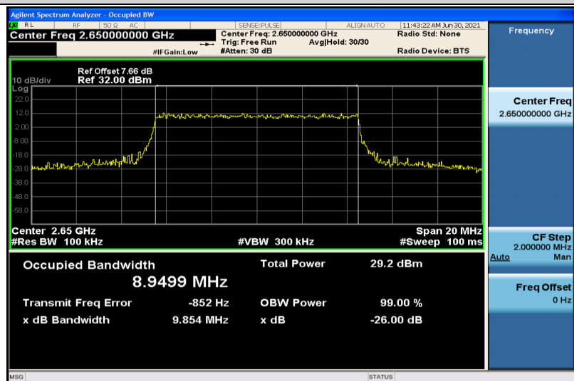
Band41-10MHz-QPSK-41190-50RB#0-8.9499
