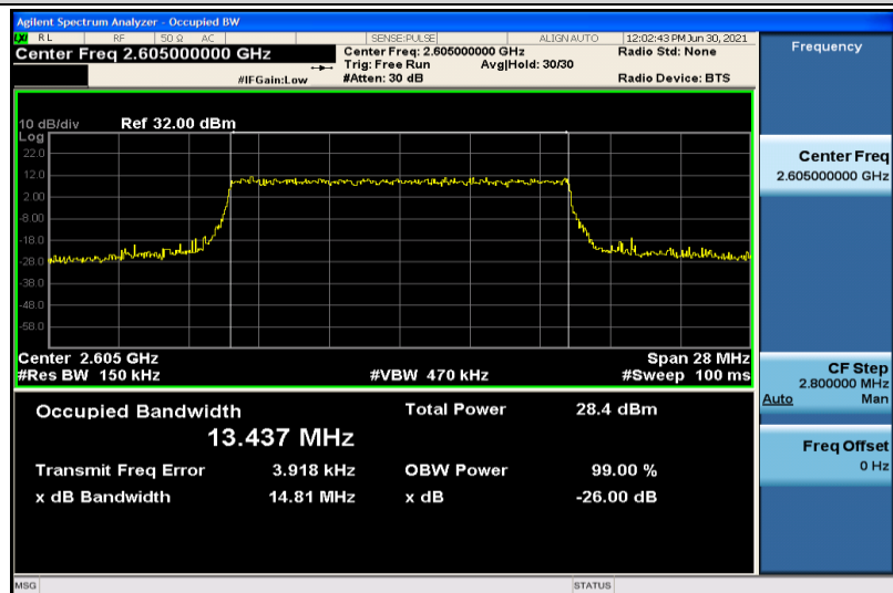
Band41-15MHz-16QAM-40740-75RB#0-13.437
