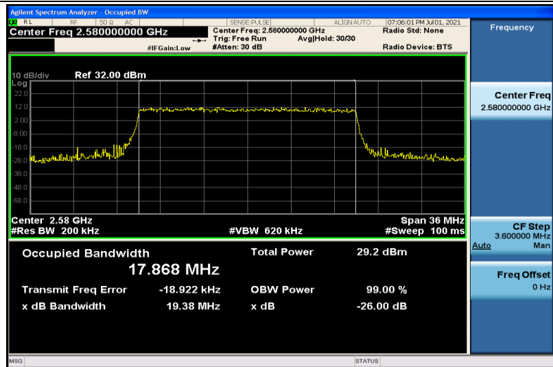
Band38-20MHz-QPSK-37850-100RB#0-17.868
