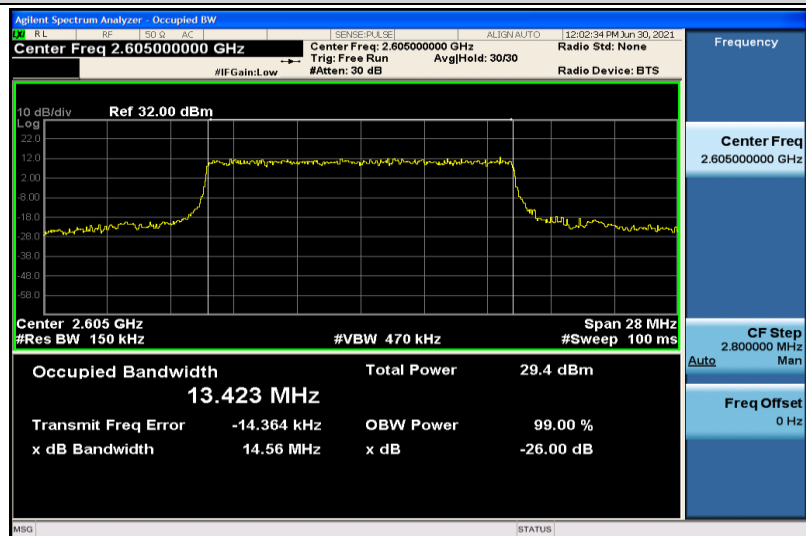
Band41-15MHz-QPSK-40740-75RB#0-13.423
