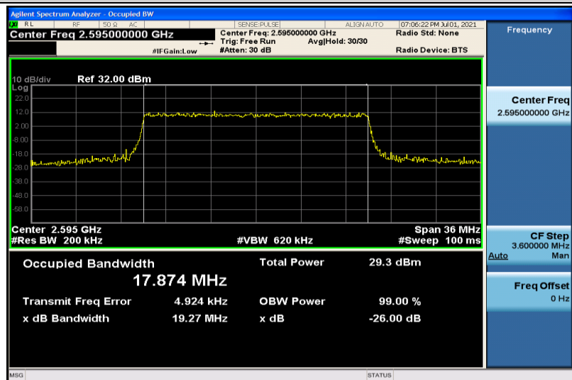
Band38-20MHz-QPSK-38000-100RB#0-17.874
