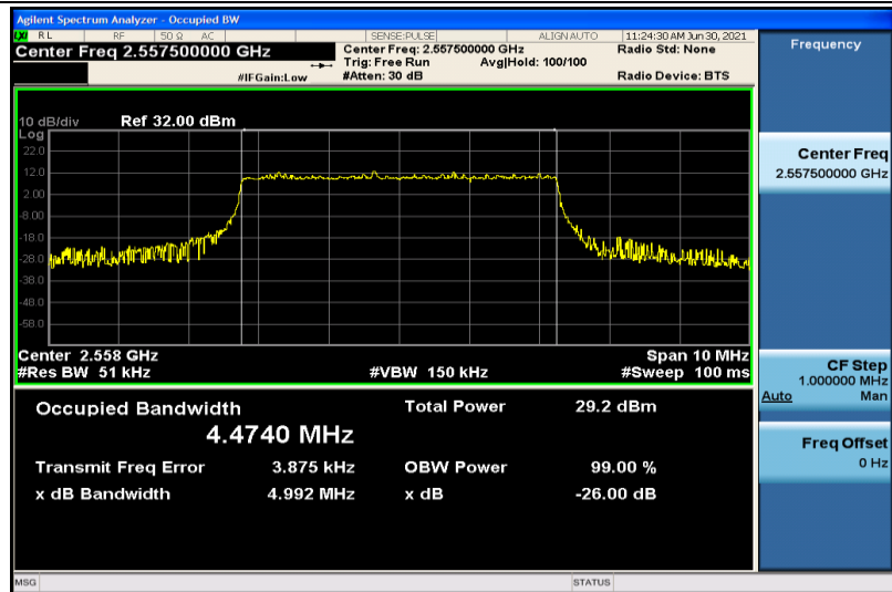
Band41-5MHz-QPSK-40265-25RB#0-4.4740
