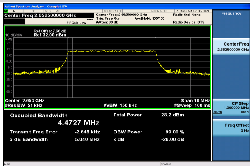
Band41-5MHz-16QAM-41215-25RB#0-4.4727
