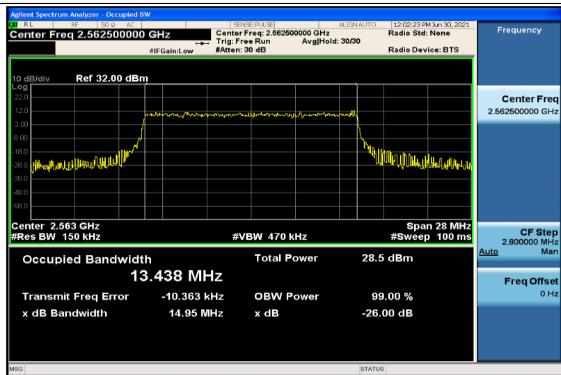
Band41-15MHz-16QAM-40315-75RB#0-13.438
