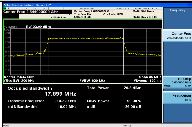
Band41-20MHz-QPSK-41140-100RB#0-17.899
