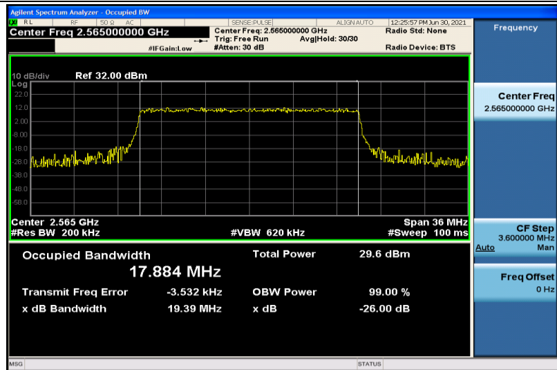
Band41-20MHz-QPSK-40340-100RB#0-17.884
