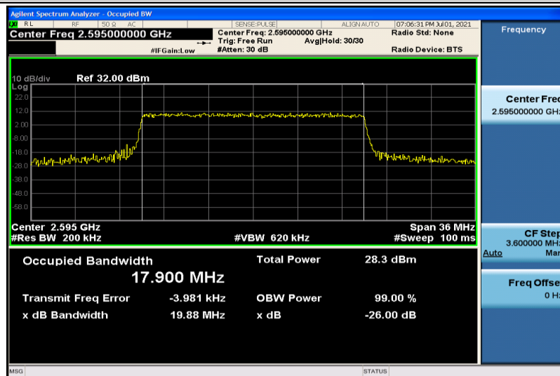
Band38-20MHz-16QAM-38000-100RB#0-17.900
