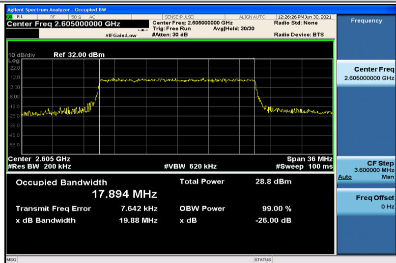
Band41-20MHz-16QAM-40740-100RB#0-17.894
