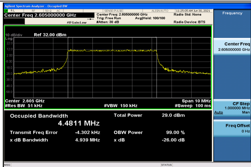
Band41-5MHz-QPSK-40740-25RB#0-4.4811
