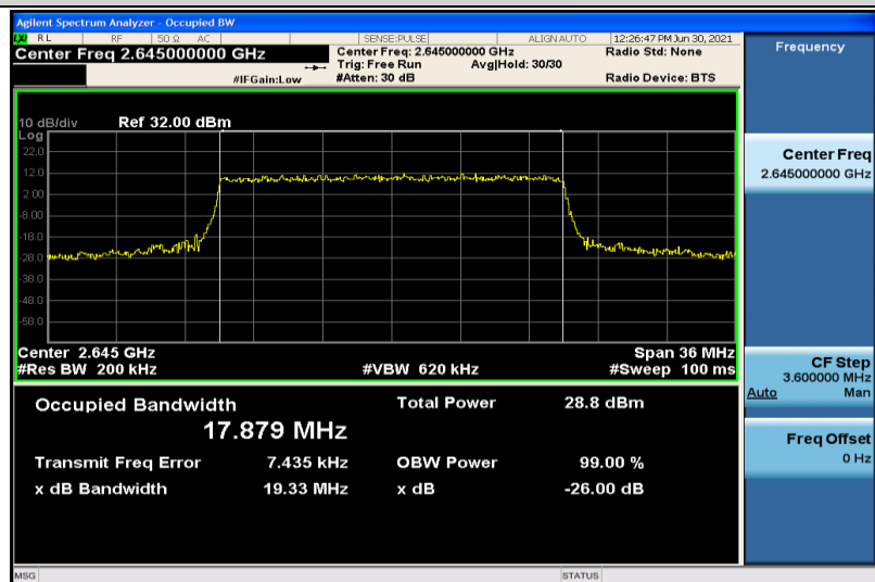
Band41-20MHz-16QAM-41140-100RB#0-17.879
