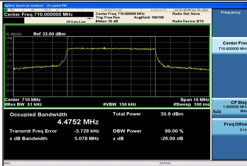
Band17-5MHz-QPSK-23790-25RB#0-4.4752
