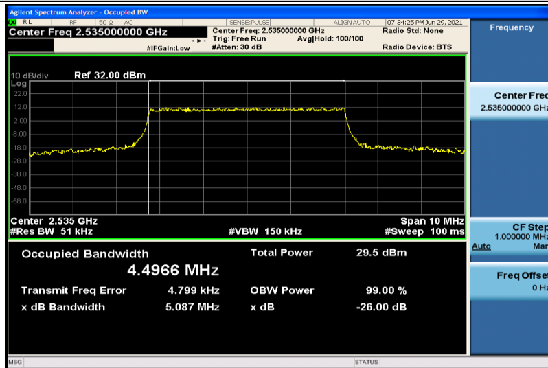
Band7-5MHz-16QAM-21100-25RB#0-4.4966
