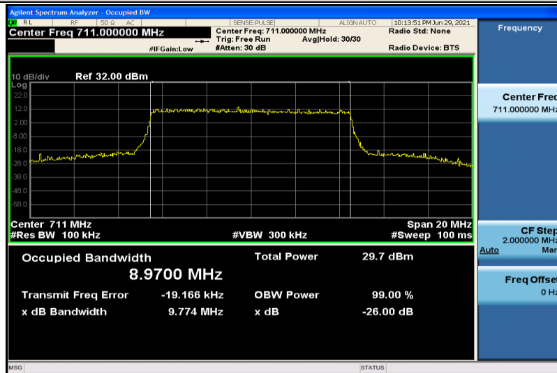
Band12-10MHz-16QAM-23130-50RB#0-8.9700
