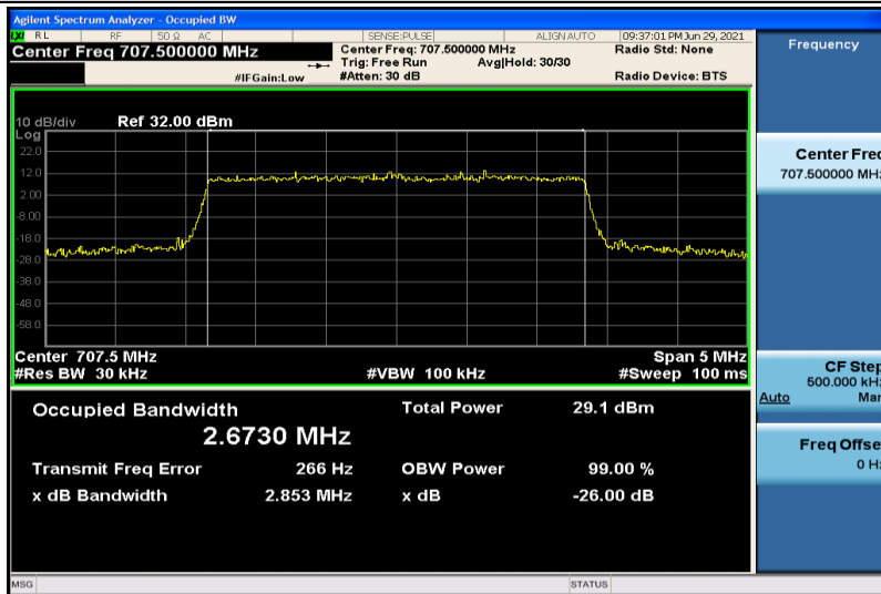
Band12-3MHz-16QAM-23095-15RB#0-2.6730
