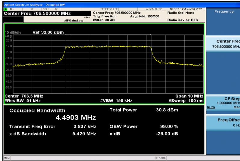
Band17-5MHz-QPSK-23755-25RB#0-4.4903
