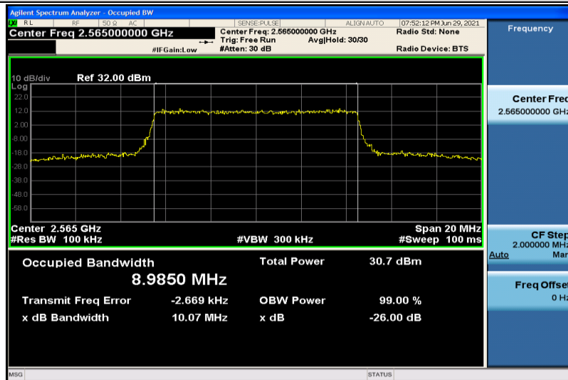
Band7-10MHz-QPSK-21400-50RB#0-8.9850
