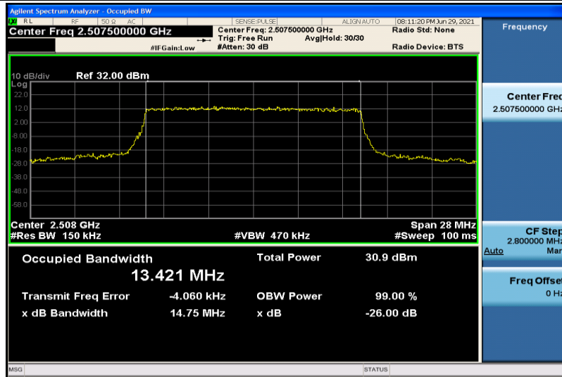
Band7-15MHz-QPSK-20825-75RB#0-13.421
