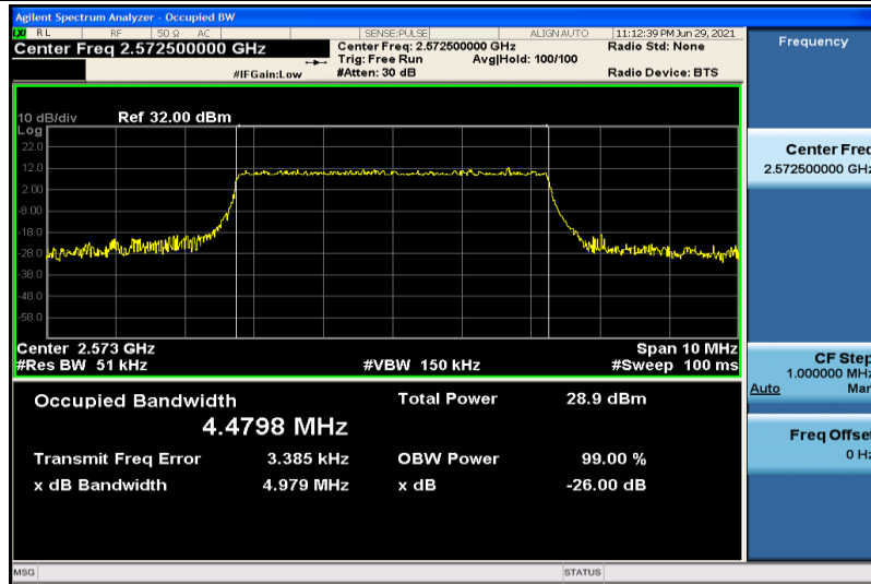
Band38-5MHz-16QAM-37775-25RB#0-4.4798
