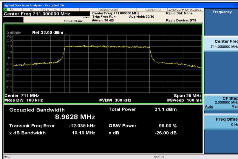
Band17-10MHz-QPSK-23800-50RB#0-8.9628
