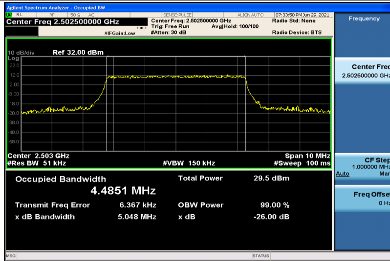
Band7-5MHz-16QAM-20775-25RB#0-4.4851
