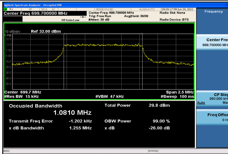
Band12-1.4MHz-QPSK-23017-6RB#0-1.0810
