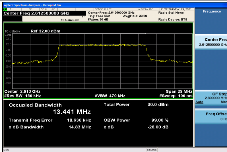
Band38-15MHz-QPSK-38175-75RB#0-13.441
