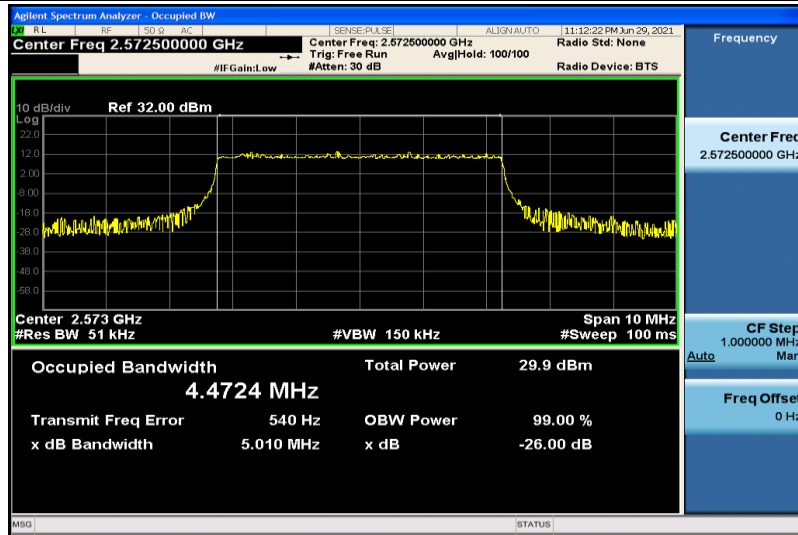
Band38-5MHz-QPSK-37775-25RB#0-4.4724
