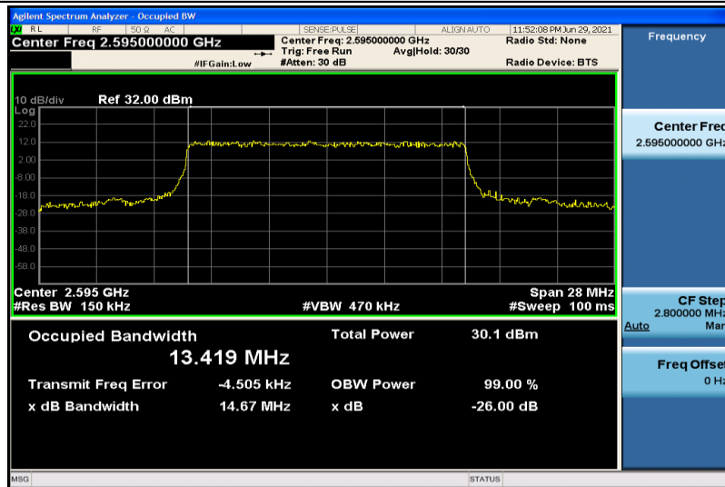
Band38-15MHz-QPSK-38000-75RB#0-13.419
