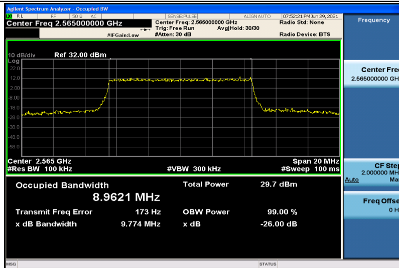
Band7-10MHz-16QAM-21400-50RB#0-8.9621
