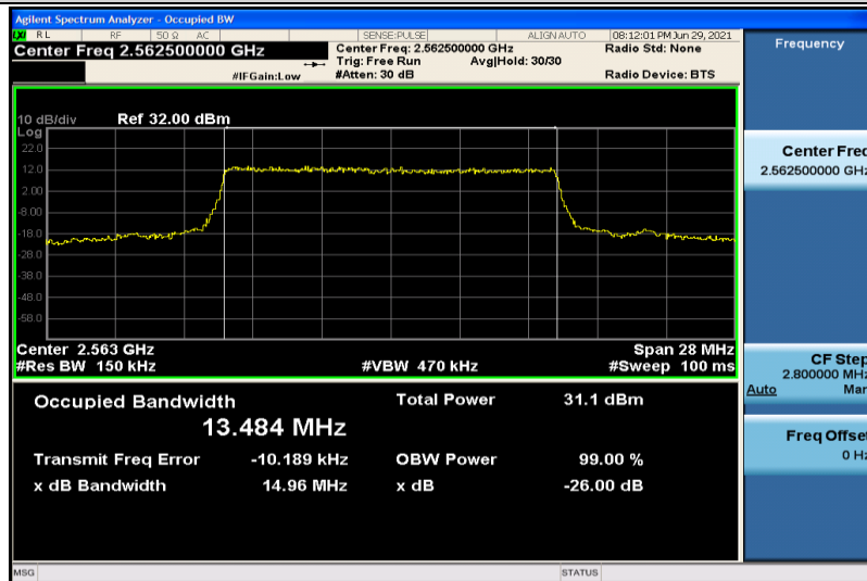
Band7-15MHz-QPSK-21375-75RB#0-13.484
