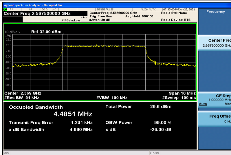
Band7-5MHz-16QAM-21425-25RB#0-4.4851
