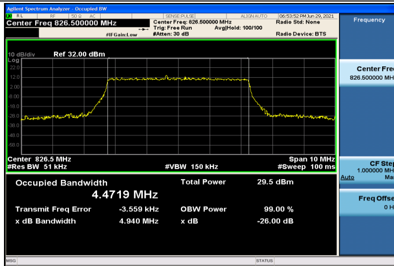
Band5-5MHz-16QAM-20425-25RB#0-4.4719
