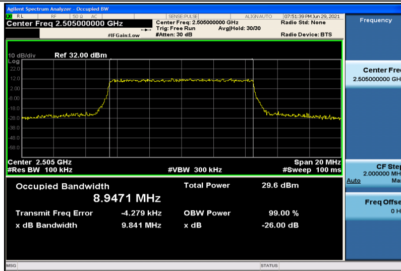
Band7-10MHz-16QAM-20800-50RB#0-8.9471
