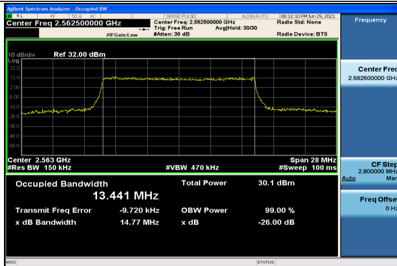
Band7-15MHz-16QAM-21375-75RB#0-13.441
