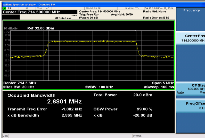
Band12-3MHz-16QAM-23165-15RB#0-2.6801
