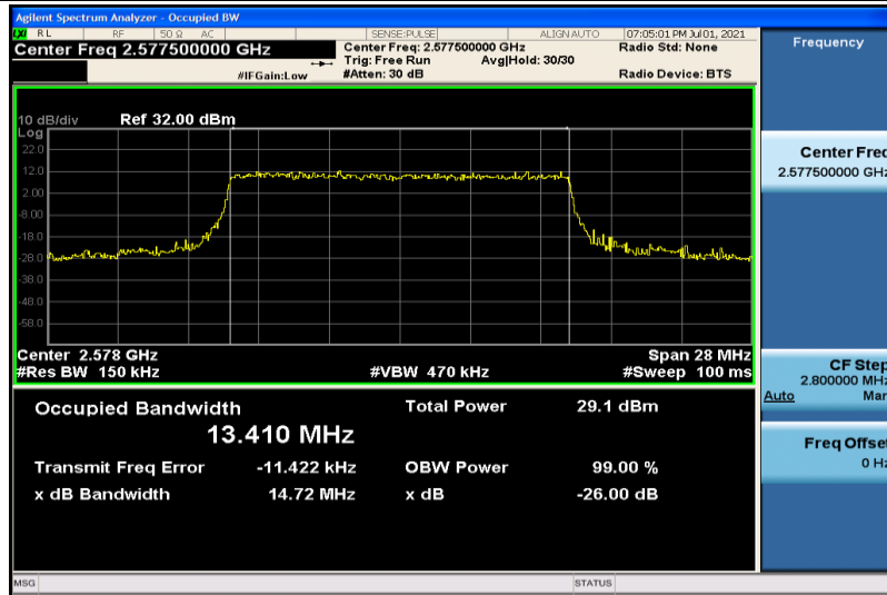
Band38-15MHz-QPSK-37825-75RB#0-13.410
