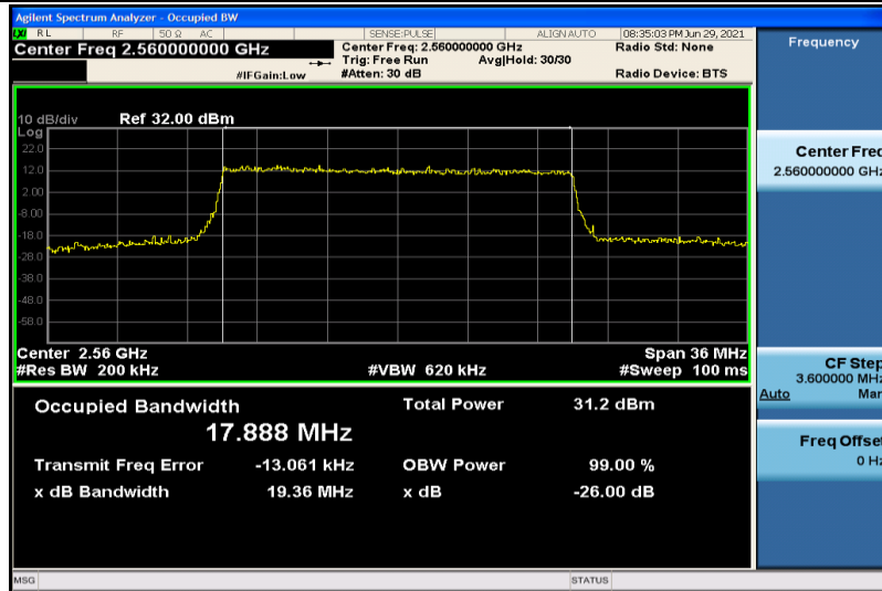
Band7-20MHz-QPSK-21350-100RB#0-17.888
