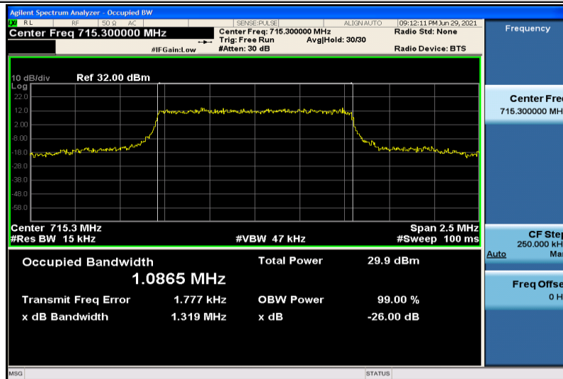
Band12-1.4MHz-QPSK-23173-6RB#0-1.0865
