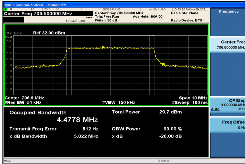
Band17-5MHz-16QAM-23755-25RB#0-4.4778
