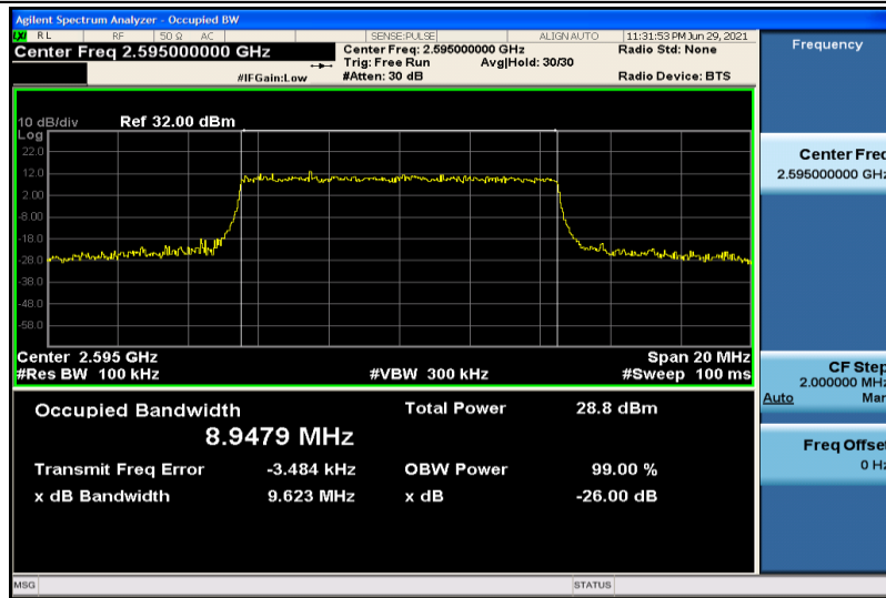
Band38-10MHz-16QAM-38000-50RB#0-8.9479
