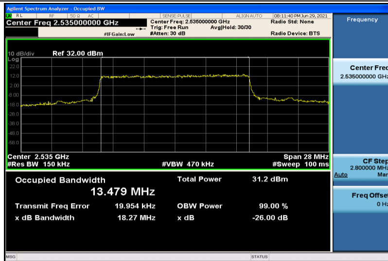
Band7-15MHz-QPSK-21100-75RB#0-13.479
