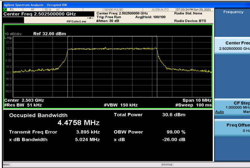
Band7-5MHz-QPSK-20775-25RB#0-4.4758
