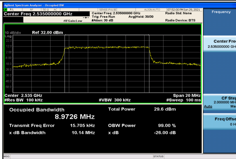
Band7-10MHz-16QAM-21100-50RB#0-8.9726
