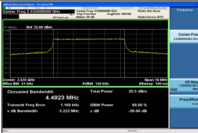
Band7-5MHz-QPSK-21100-25RB#0-4.4923
