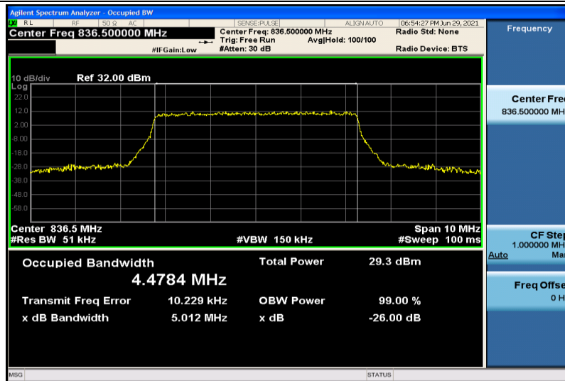
Band5-5MHz-16QAM-20525-25RB#0-4.4784
