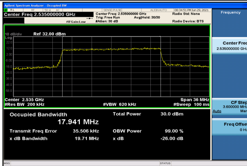
Band7-20MHz-16QAM-21100-100RB#0-17.941
