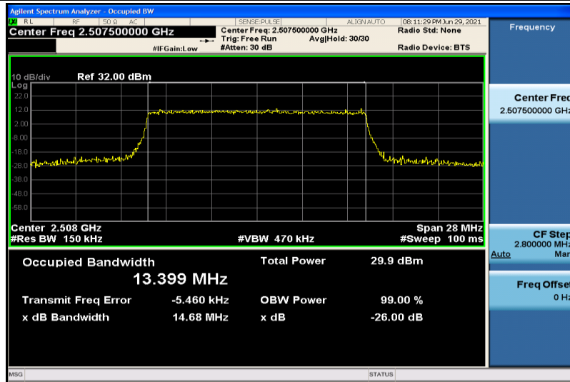
Band7-15MHz-16QAM-20825-75RB#0-13.399
