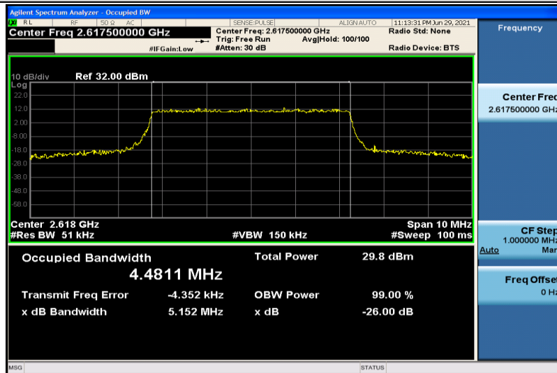
Band38-5MHz-QPSK-38225-25RB#0-4.4811
