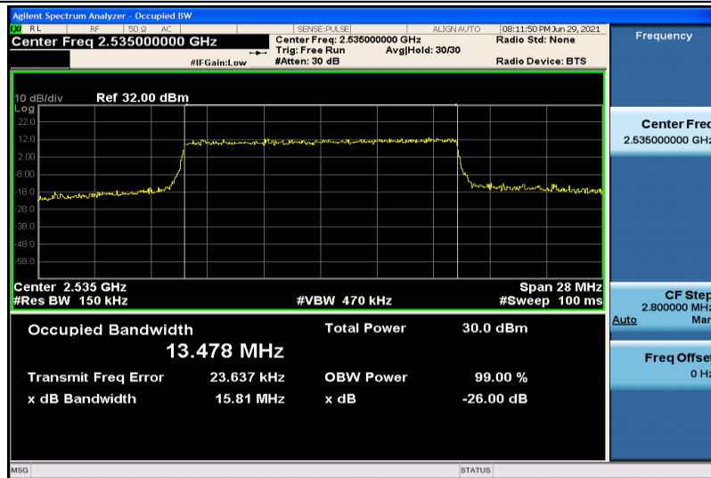
Band7-15MHz-16QAM-21100-75RB#0-13.478
