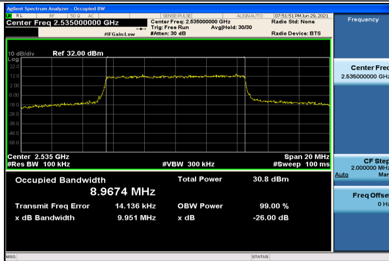
Band7-10MHz-QPSK-21100-50RB#0-8.9674
