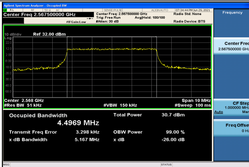
Band7-5MHz-QPSK-21425-25RB#0-4.4969
