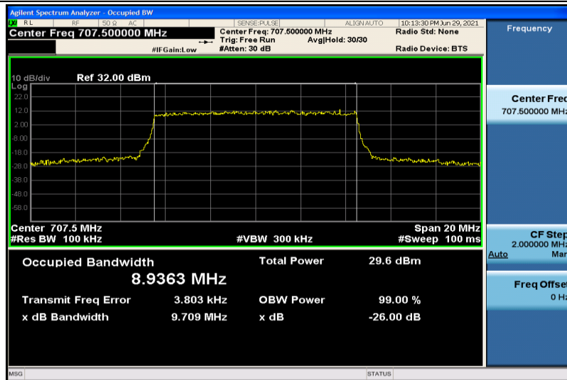
Band12-10MHz-16QAM-23095-50RB#0-8.9363
