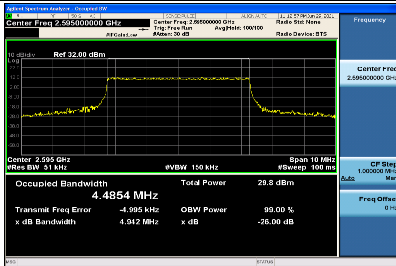
Band38-5MHz-QPSK-38000-25RB#0-4.4854
