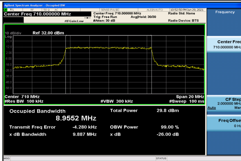
Band17-10MHz-16QAM-23790-50RB#0-8.9552
