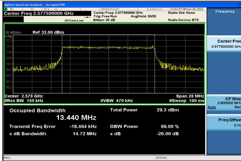
Band38-15MHz-16QAM-37825-75RB#0-13.440
