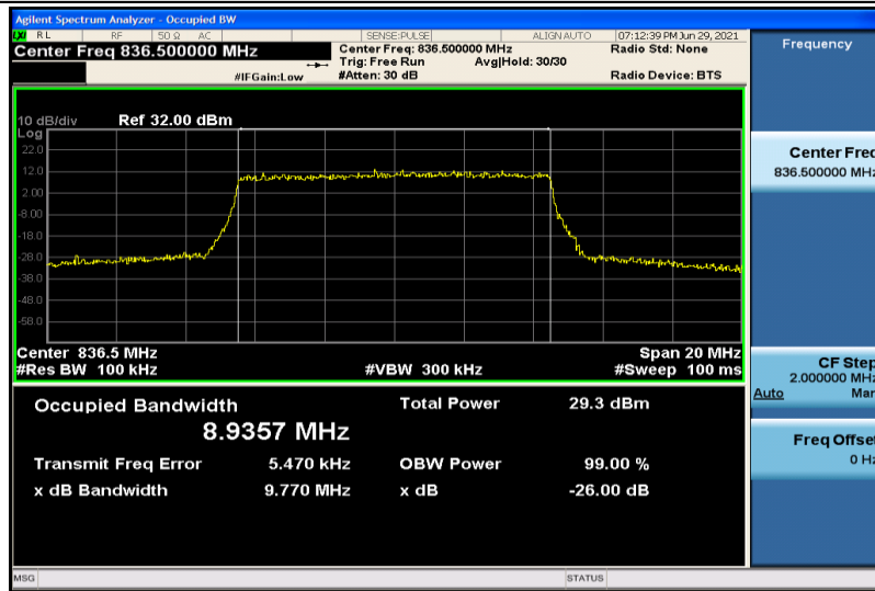
Band5-10MHz-16QAM-20525-50RB#0-8.9357
