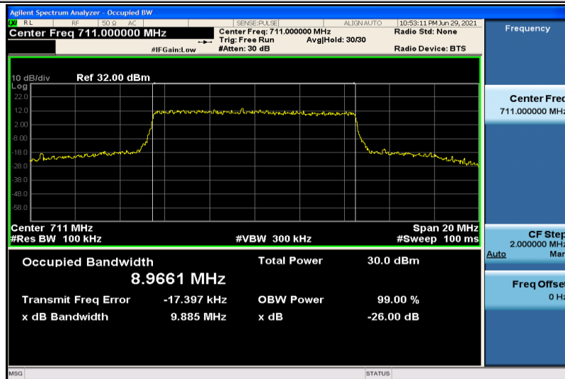
Band17-10MHz-16QAM-23800-50RB#0-8.9661
