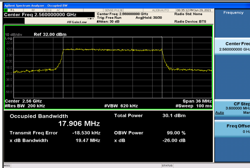
Band7-20MHz-16QAM-21350-100RB#0-17.906
