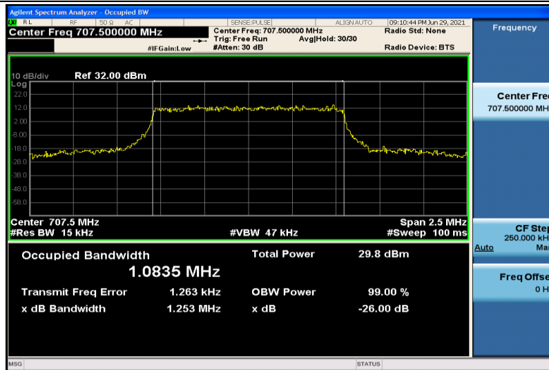
Band12-1.4MHz-QPSK-23095-6RB#0-1.0835
