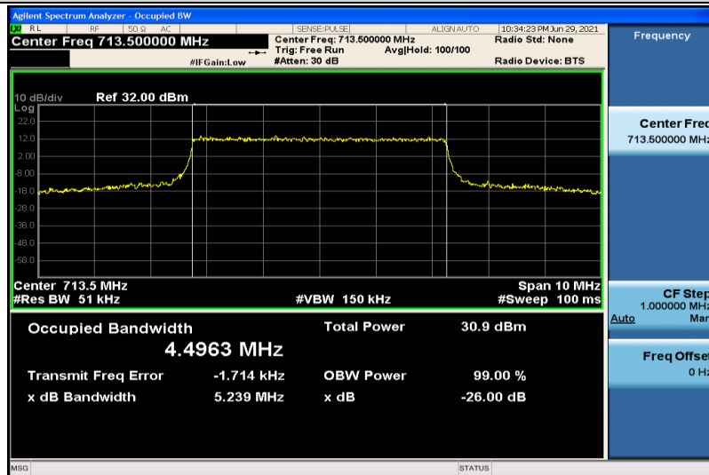
Band17-5MHz-QPSK-23825-25RB#0-4.4963
