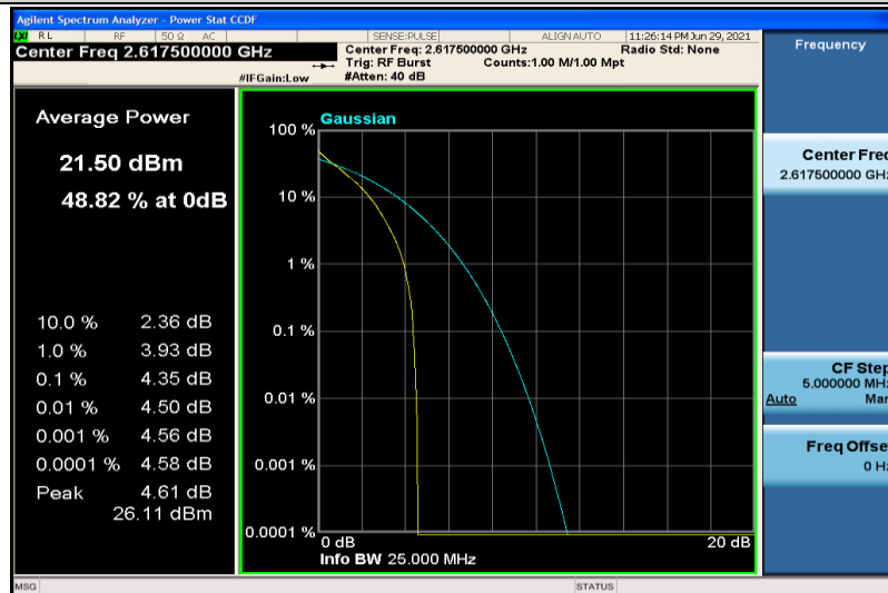
Band38-5MHz-QPSK-38225-25RB#0
