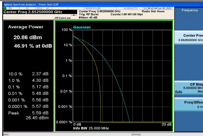
Band41-5MHz-QPSK-41215-25RB#0
