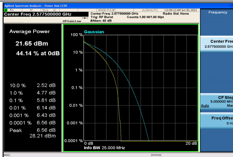
Band38-15MHz-QPSK-37825-5RB#0
