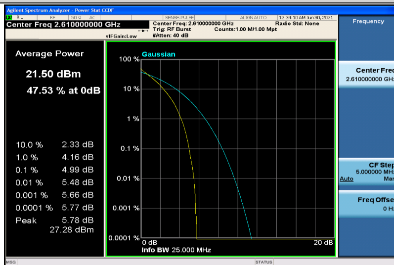
Band38-20MHz-QPSK-38150-100RB#0
