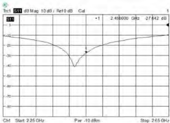
Return loss
