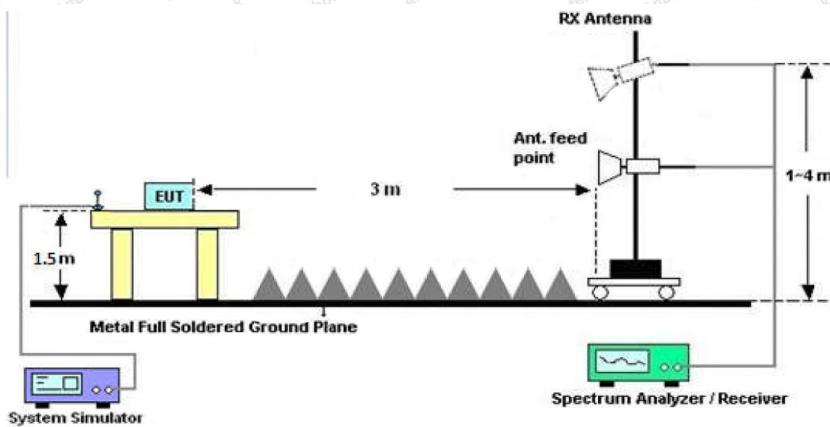
Figure 3. Above 1 GHz
