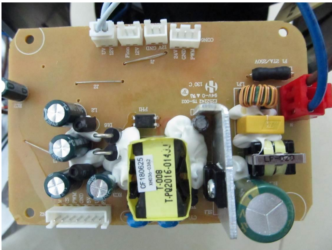
Power board
