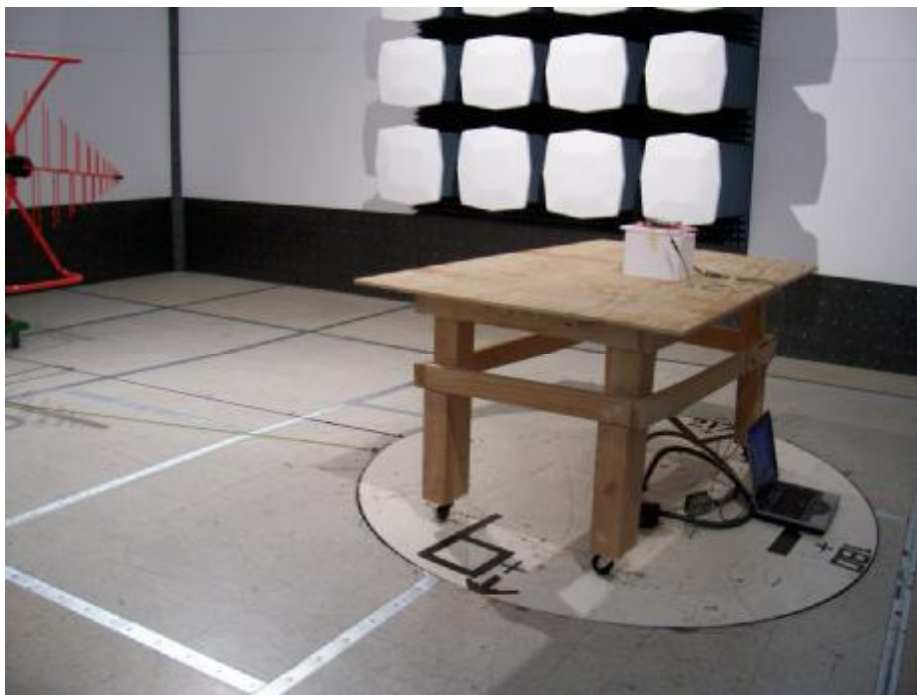
Radiated Emissions below 1GHz Setup
