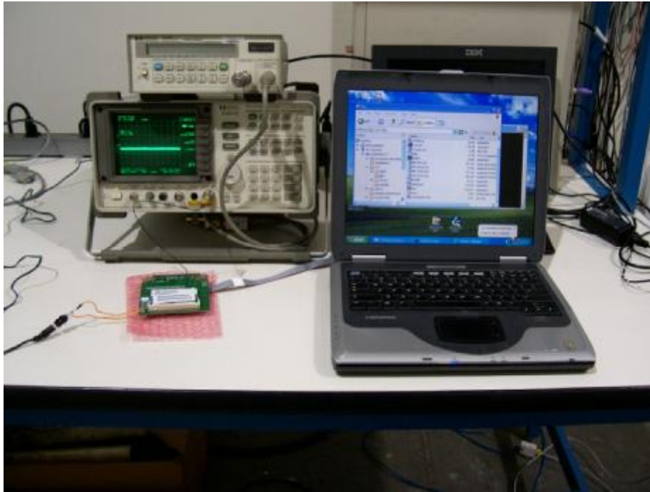
Conducted Measurement Setup
