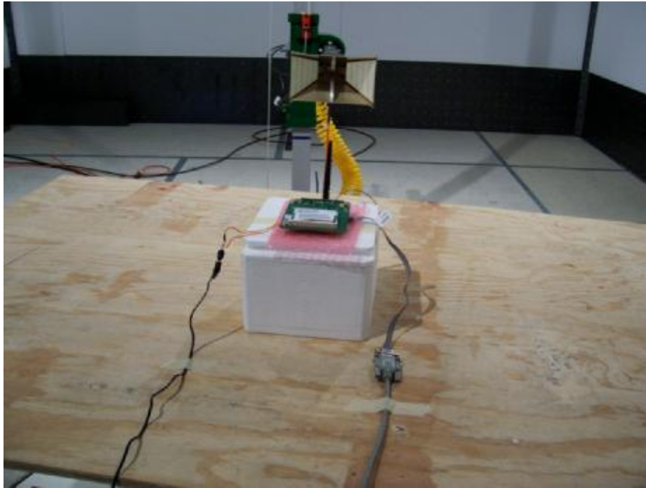
Radiated Emissions above 1GHz Setup
