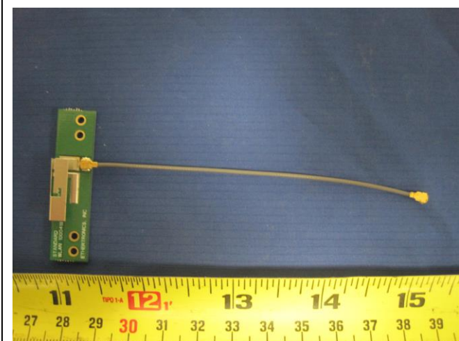
Antenna – Top View (Embedded antenna)
