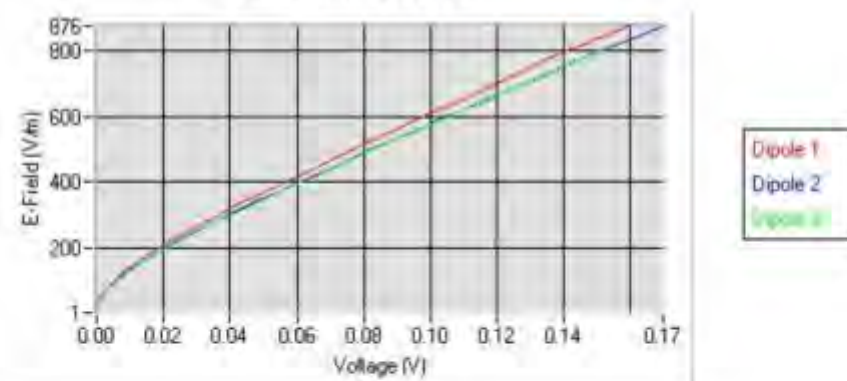
Calibration curves
