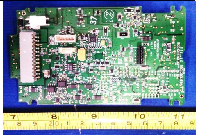
PCBA2 - Front View
