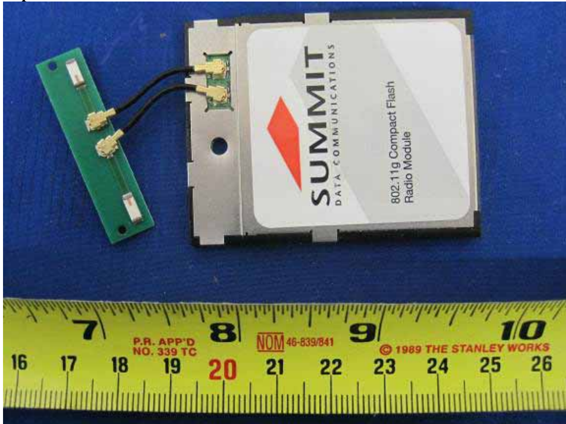
Bottom View
