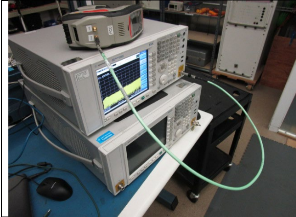
Conducted RF Emissions
