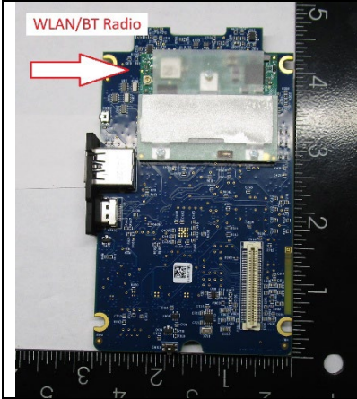
WLAN/BT Radio Location
