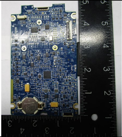
Underside WLAN/BT Radio Location
