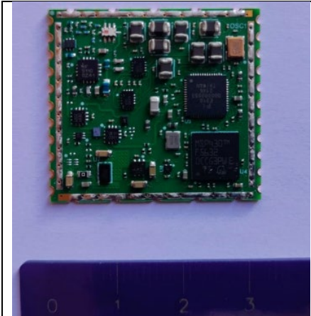
Radio – Shield Removed
