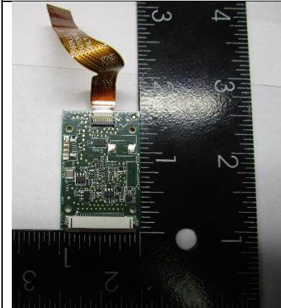
WLAN/BT Antenna
