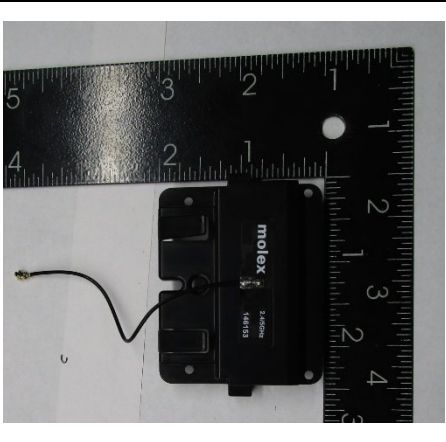
WLAN/BT Antenna
