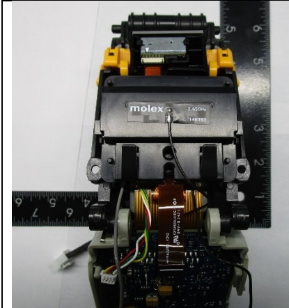
WLAN/BT Antenna
