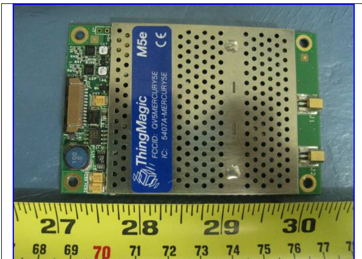
EUT (9906): RF Module PCBA Component View (Cover On)
