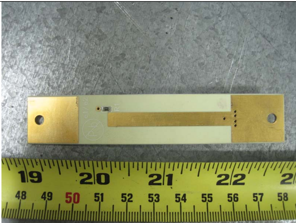
EUT (9906): UHF RFID Antenna Component View
