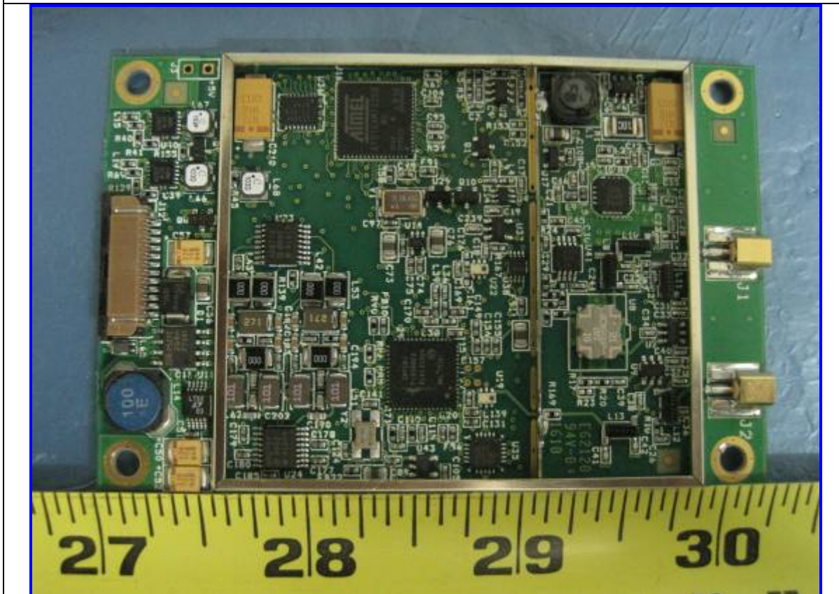
EUT (9906): RF Module PCBA Component View (Cover Off)
