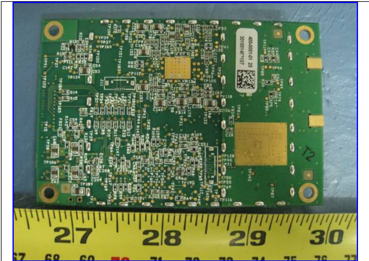
EUT (9906): RF Module PCBA Solder View
