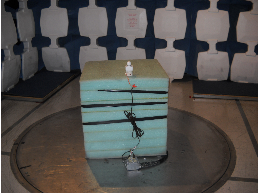
Radiated Emissions
