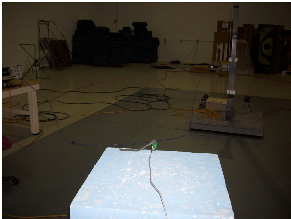
Certification Radiated Measurements above 1GHz - OATS
