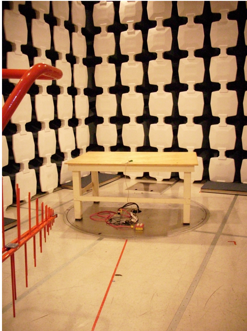
Radiated Emissions below 1GHz – Anechoic Chamber
