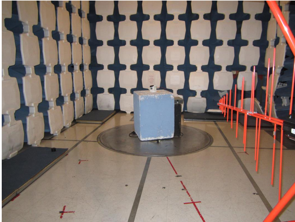
EMI-Radiated – Fundamental Measurement, EMI Spurious, Occupied BW
