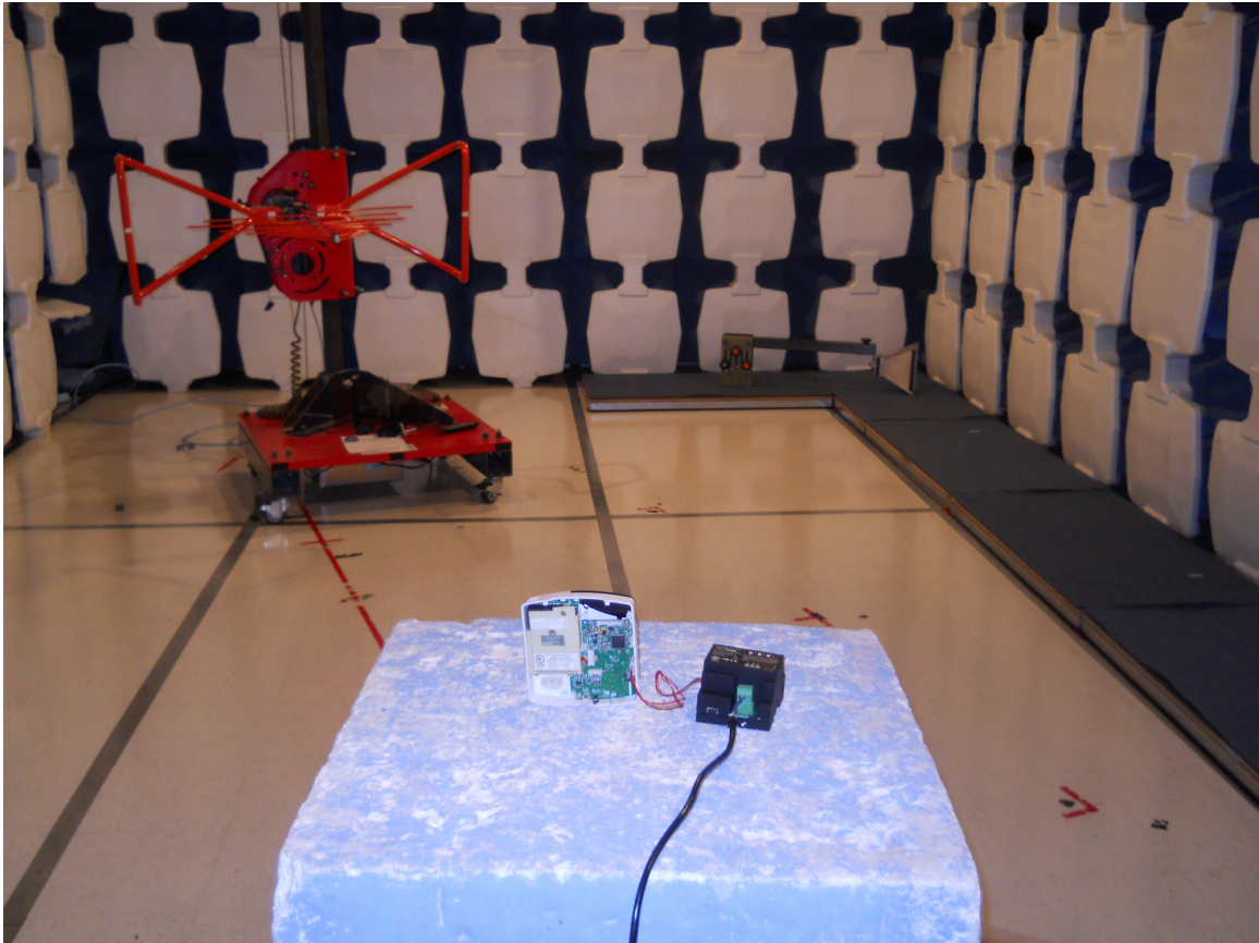
EMI Radiated
