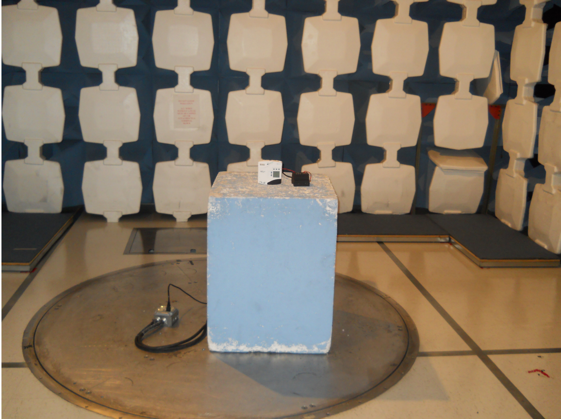
EMI Radiated
