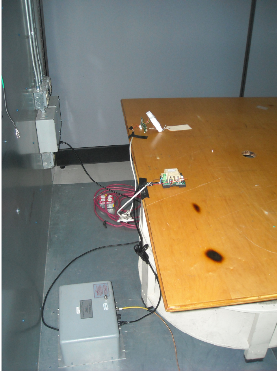
Conducted Emissions - Back
