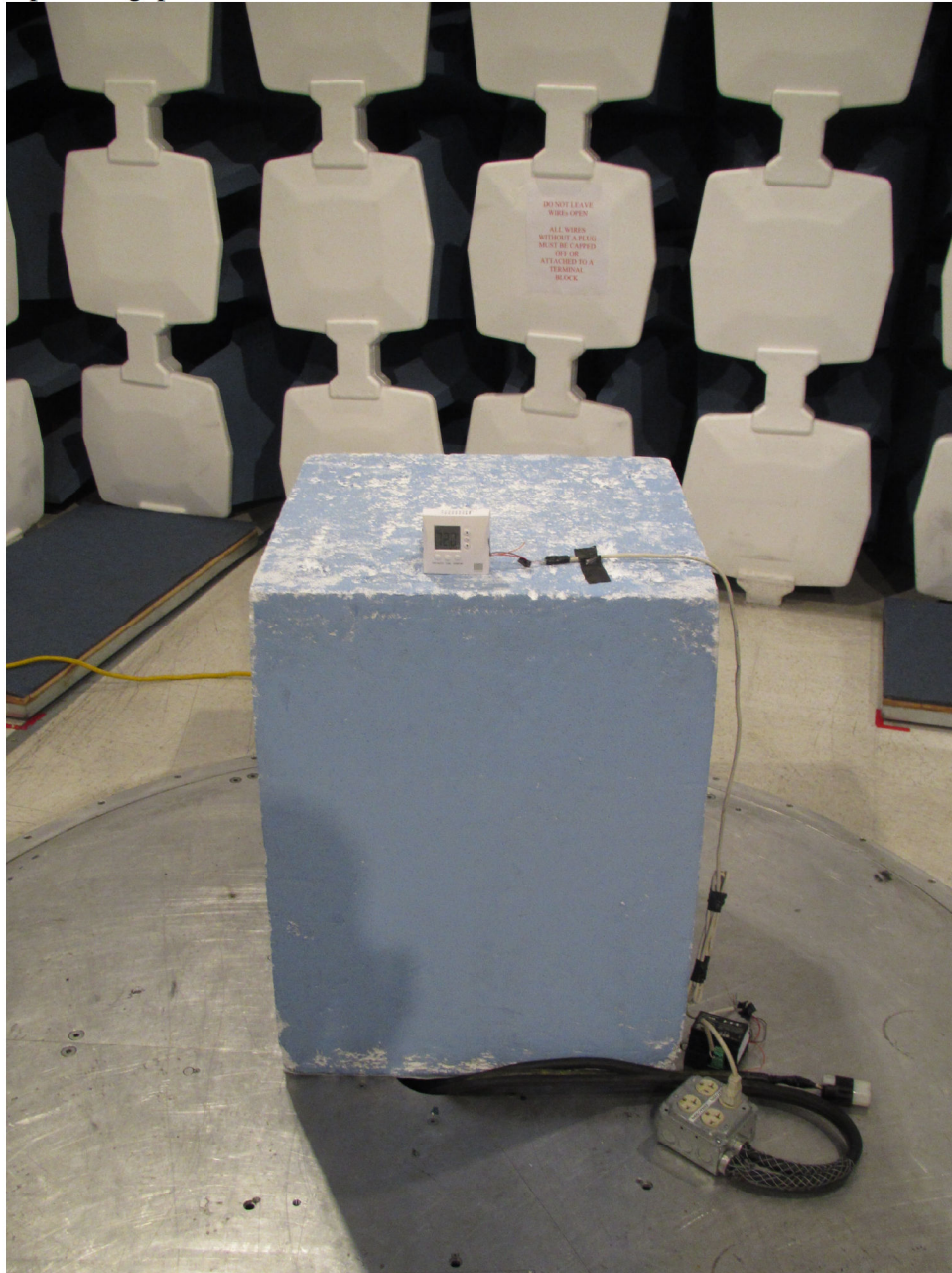
Radiated Emissions – Front
