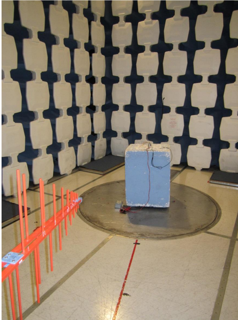
Radiated Emissions – Rear View
