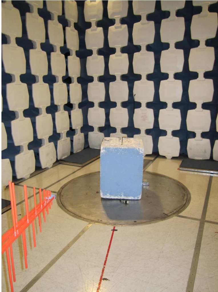
Radiated Emissions – Front View
