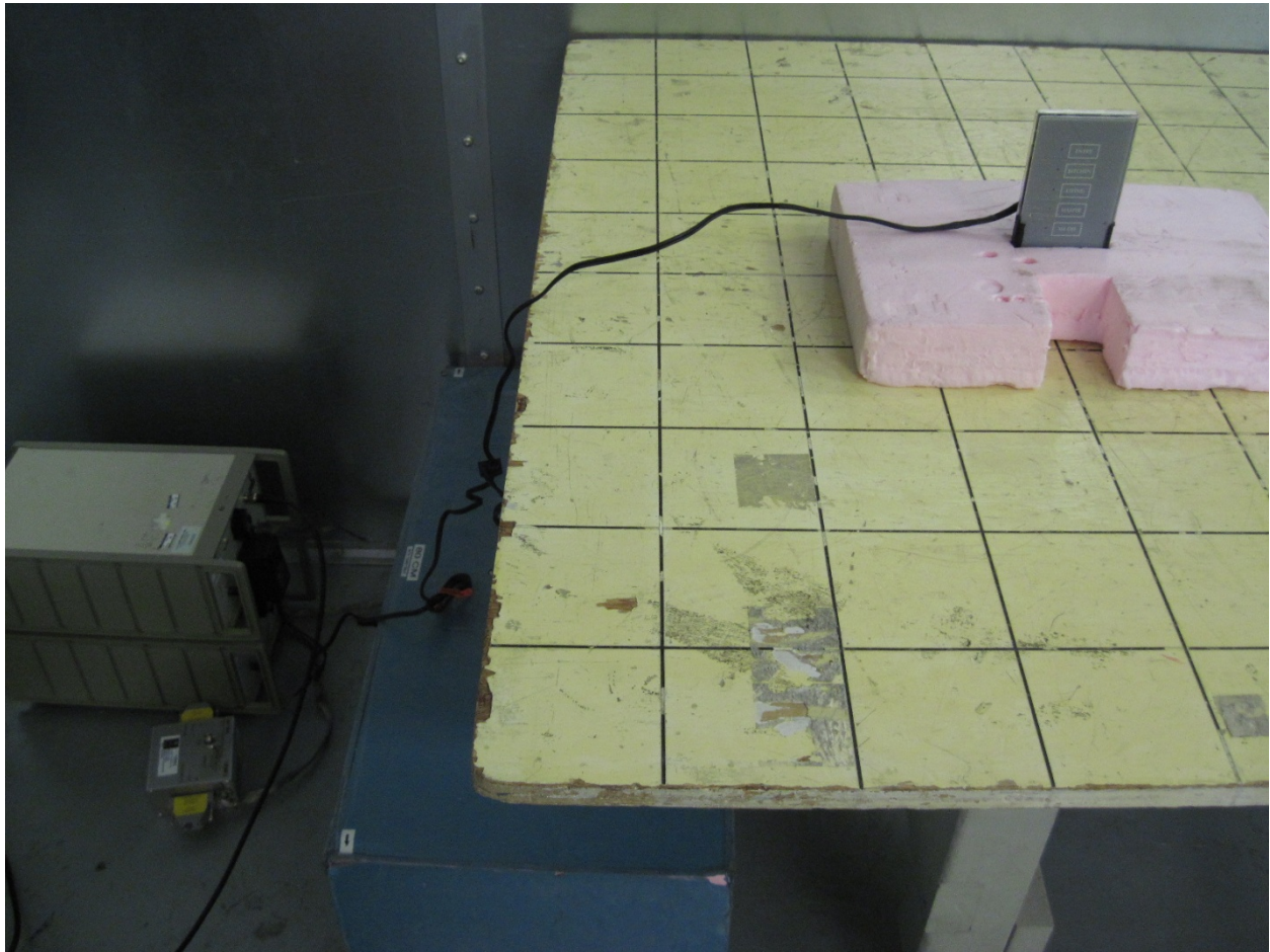
Conducted Emissions Test Setup Photo
