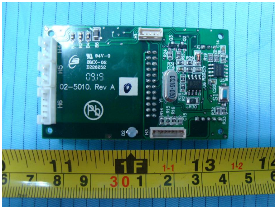
EUT – Logic Board Bottom View
