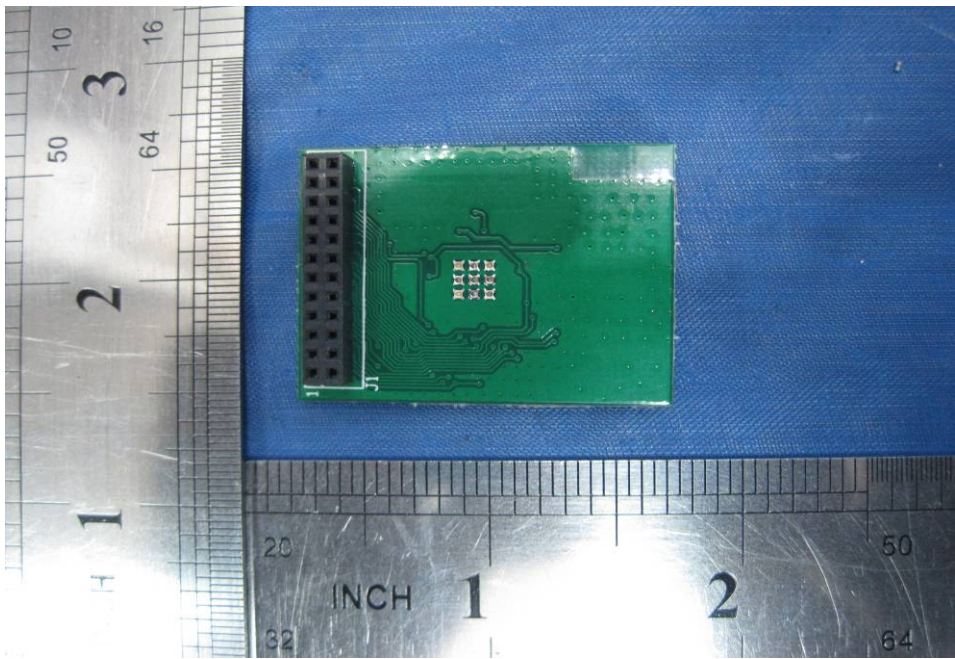
2.5PCB2 - Back View
