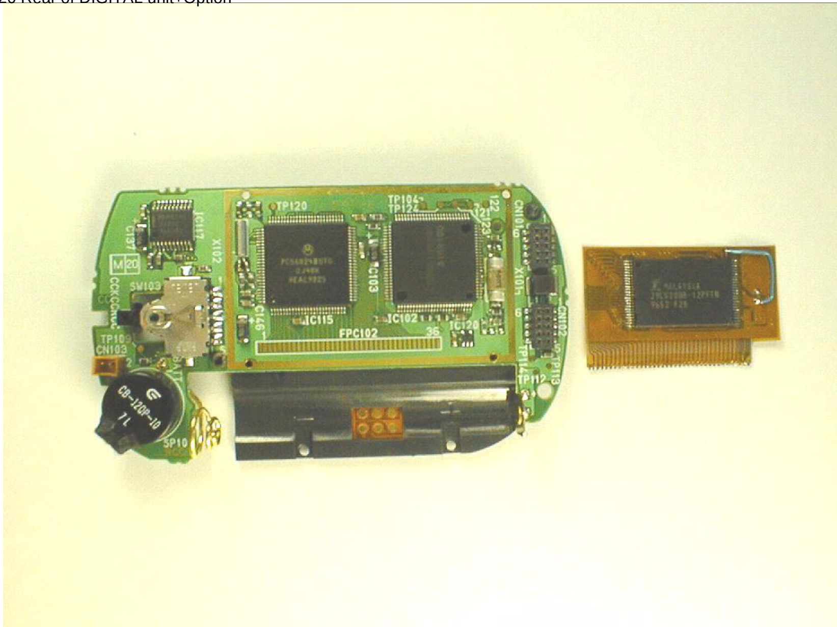
PB2320 Rear of DIGITAL unit+Option
