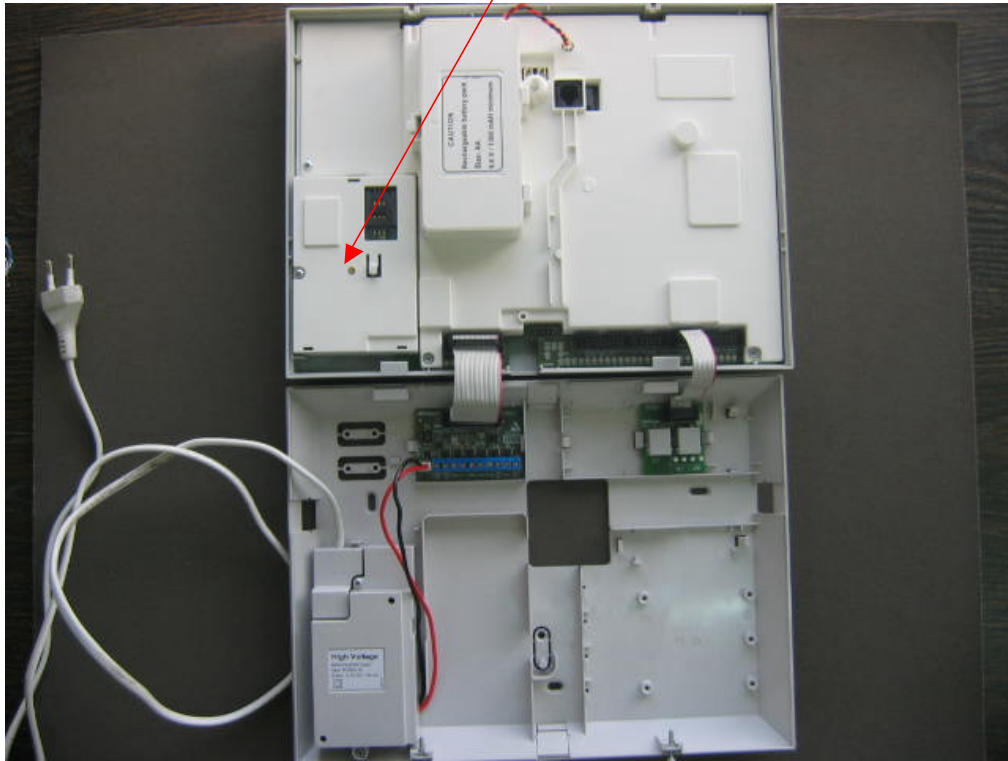
Photograph No.1 PowerMax Pro internal view with GSM module
