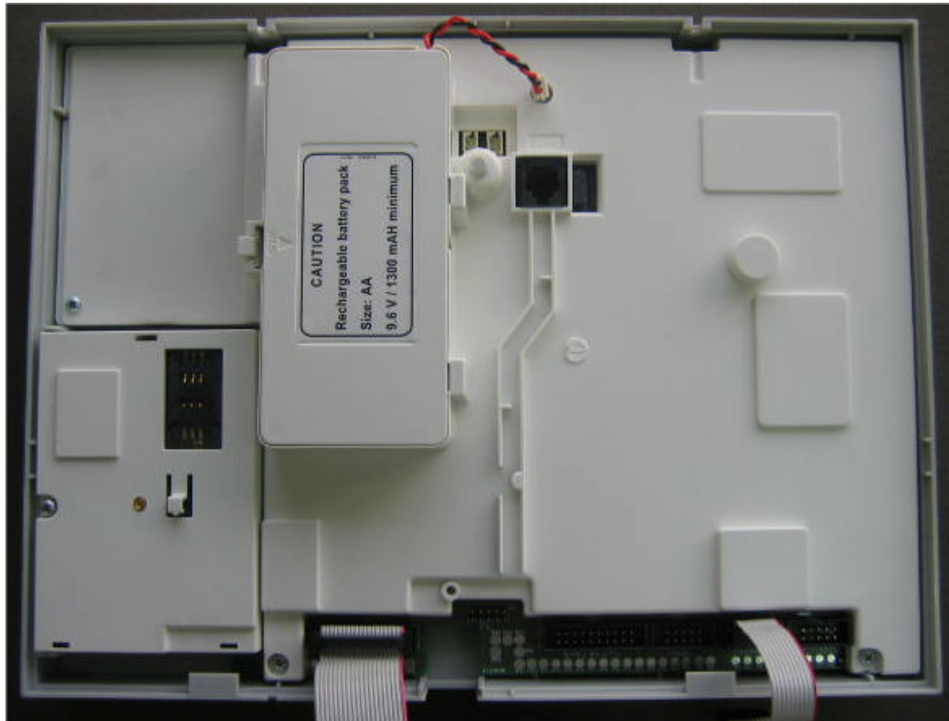
Photograph No.2 PowerMax Pro main part internal view with covers
