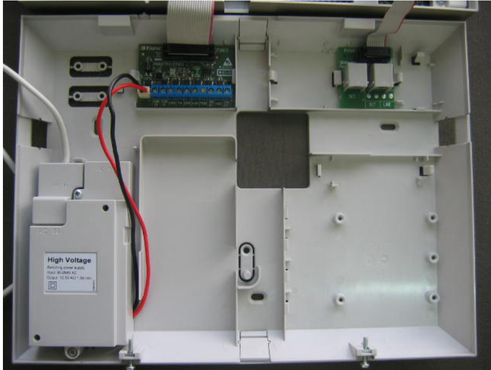
Photograph No.3 PowerMax Pro back cover internal view
