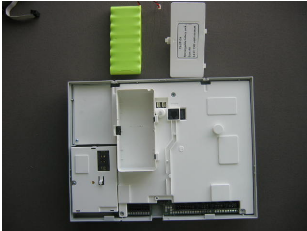
Photograph No.4 PowerMax Pro with battery pack removed
